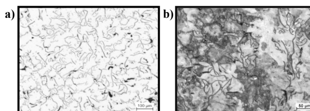
Fig. 4. Grey cast iron – material from the original brake disk; (a) size and shape of graphite precipitates – non-etched microsection; (b) microstructure of the alloy – microsection etched with Nital
