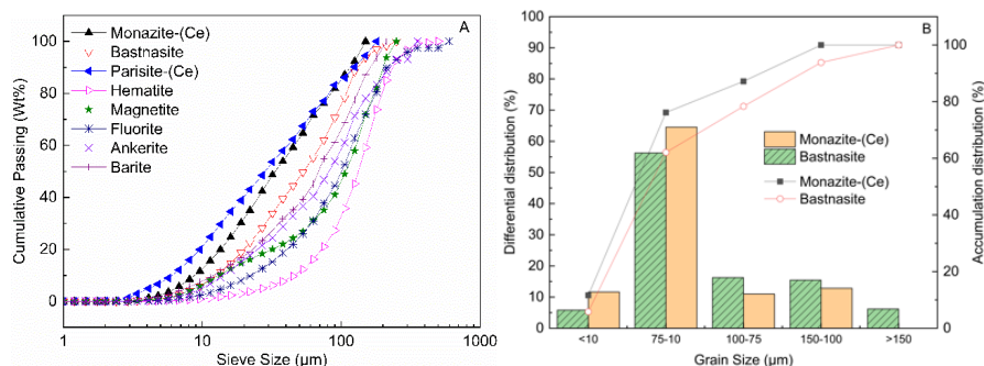
Fig. 1. Mineral grain size distribution with grinding fineness of 19.86% passing 75 \mu\text{m} A: Main minerals, B: Main rare earth minerals
