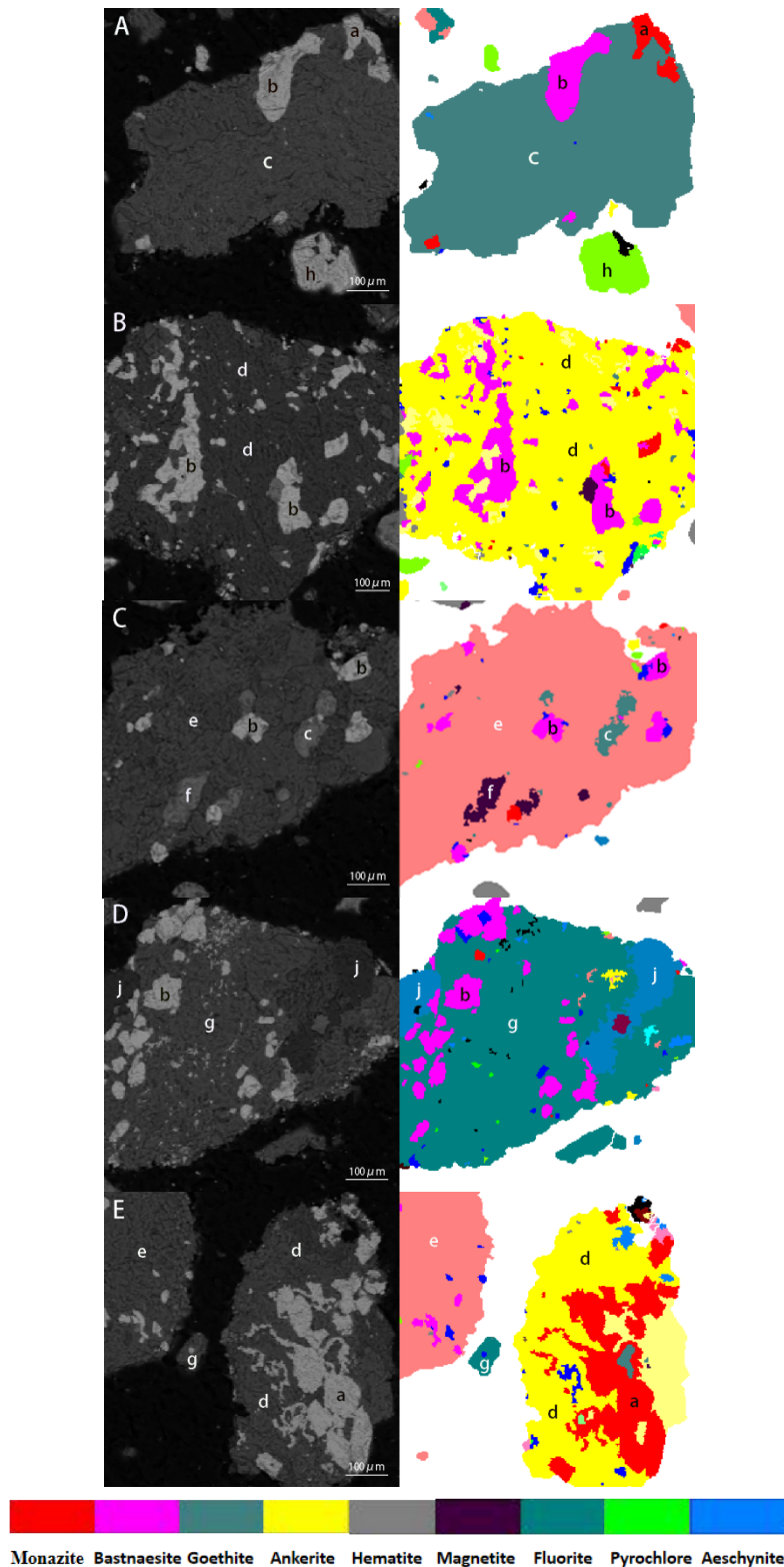
Fig. 3. BSE images and X-ray mapping with main minerals directed to false colors of Bayan Obo rare earth ores
