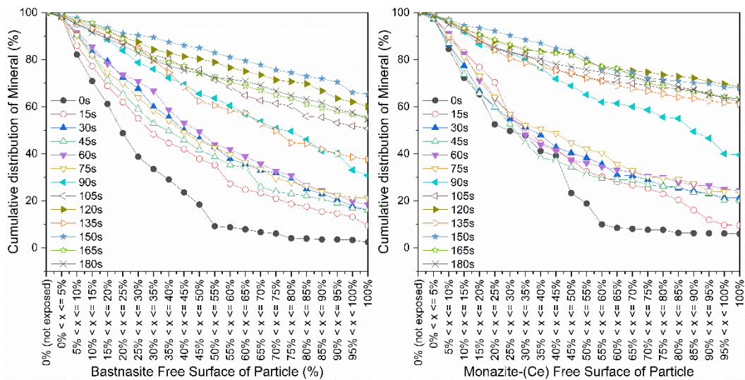
Fig. 4. Mineral liberation by free surface
