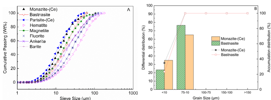
Fig. 2. Mineral grain size distribution with grinding fineness of 83.57% passing 75 \mu\text{m} A: Main minerals, B: Main rare earth minerals
