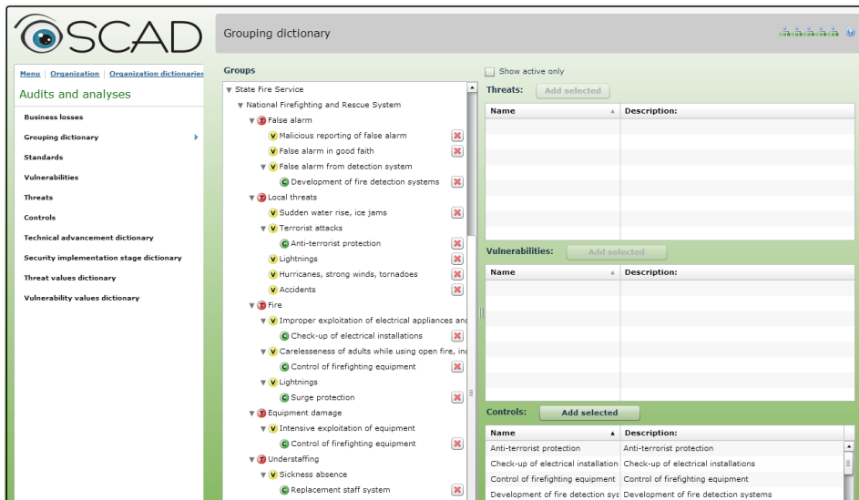
Fig. 5 OSCAD for fire protection – defining domain vocabulary Source: EMAG’s documentation, 2013
