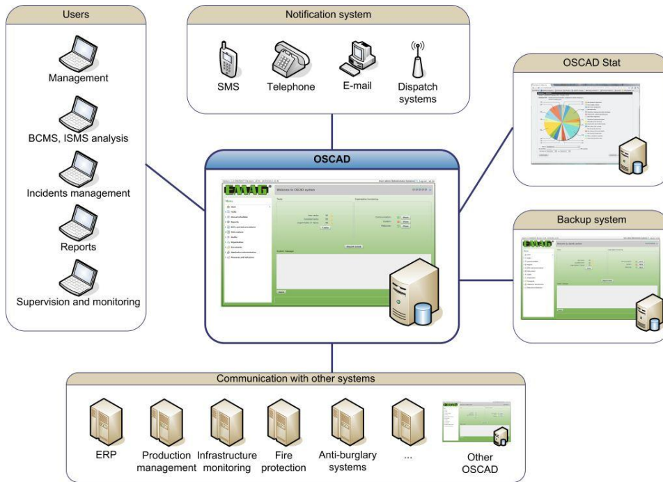
Fig. 1. Diagram of the OSCAD system Source: EMAG's documentation, 2012
