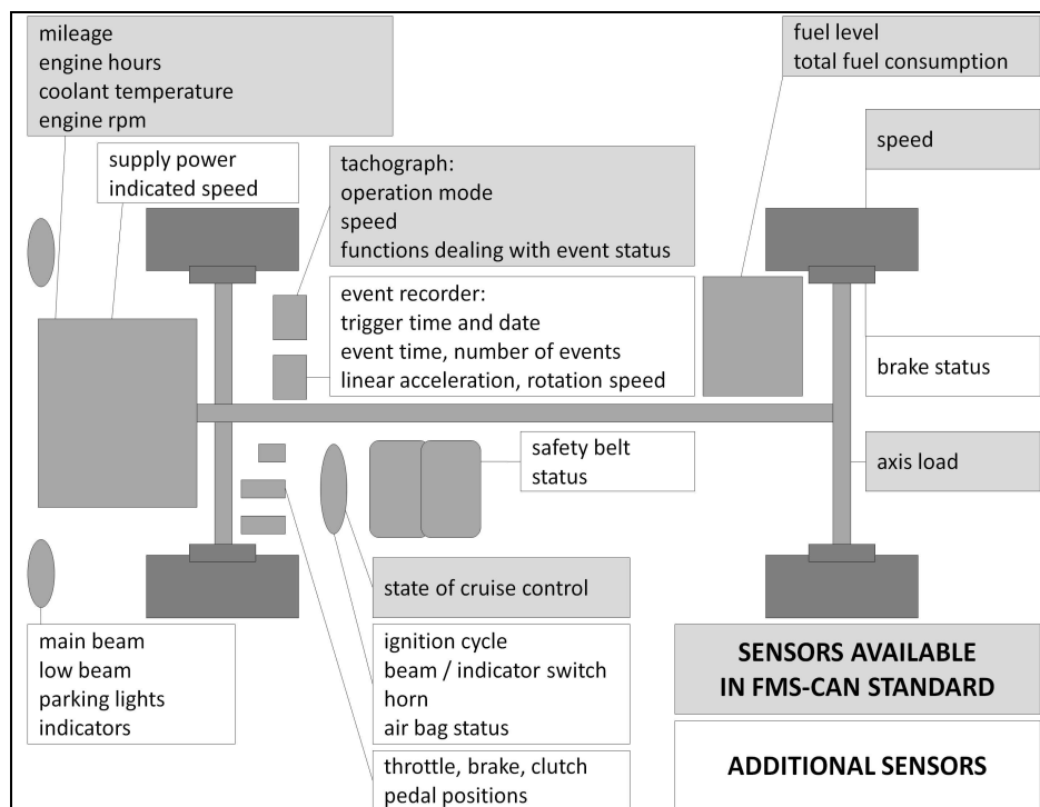
Fig. 1. Monitoring sensors in vehicle
