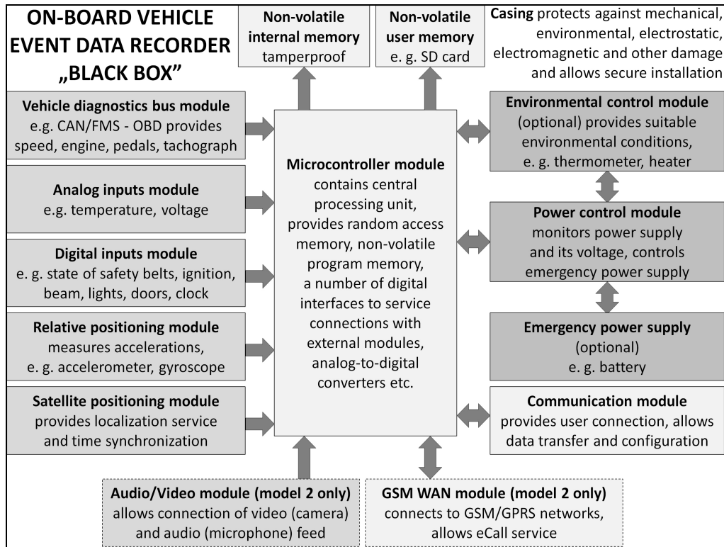
Fig. 2. On-board vehicle, event data recorder functional structure
