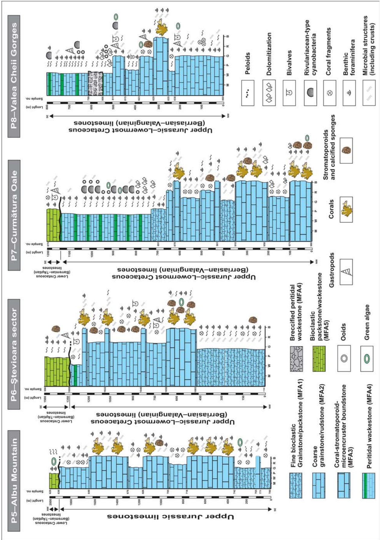
Fig. 4. General succession of the limestone deposits of the Buila-Vânturarița Massif (sections P5 to P8).
