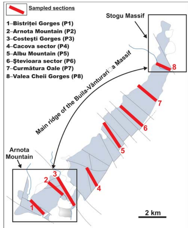
Fig. 2. Location of the sections studied.
