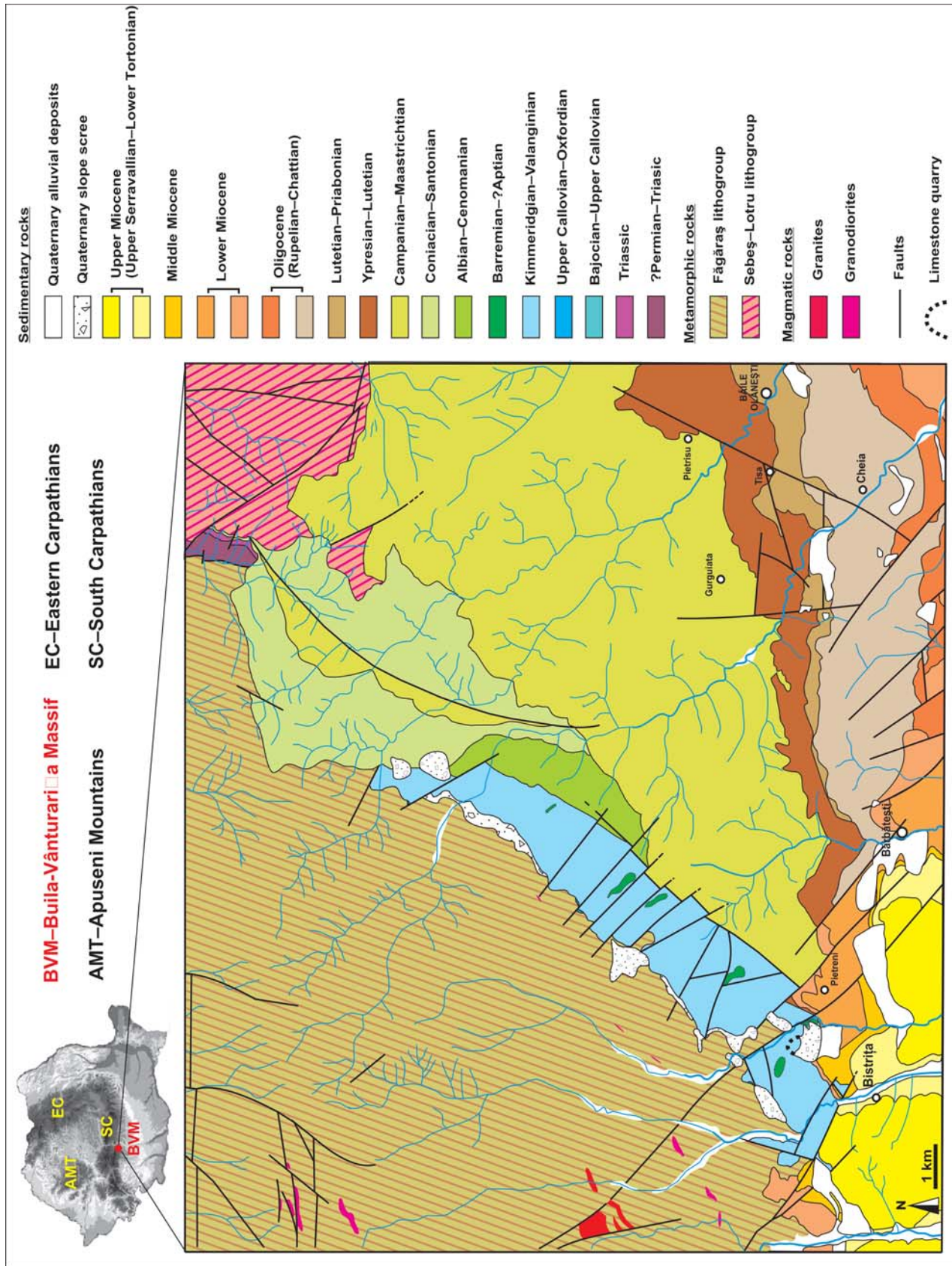
Fig. 1. Geological map of the Buila-Vânturarița Massif (modified after Lupu et al., 1978).
