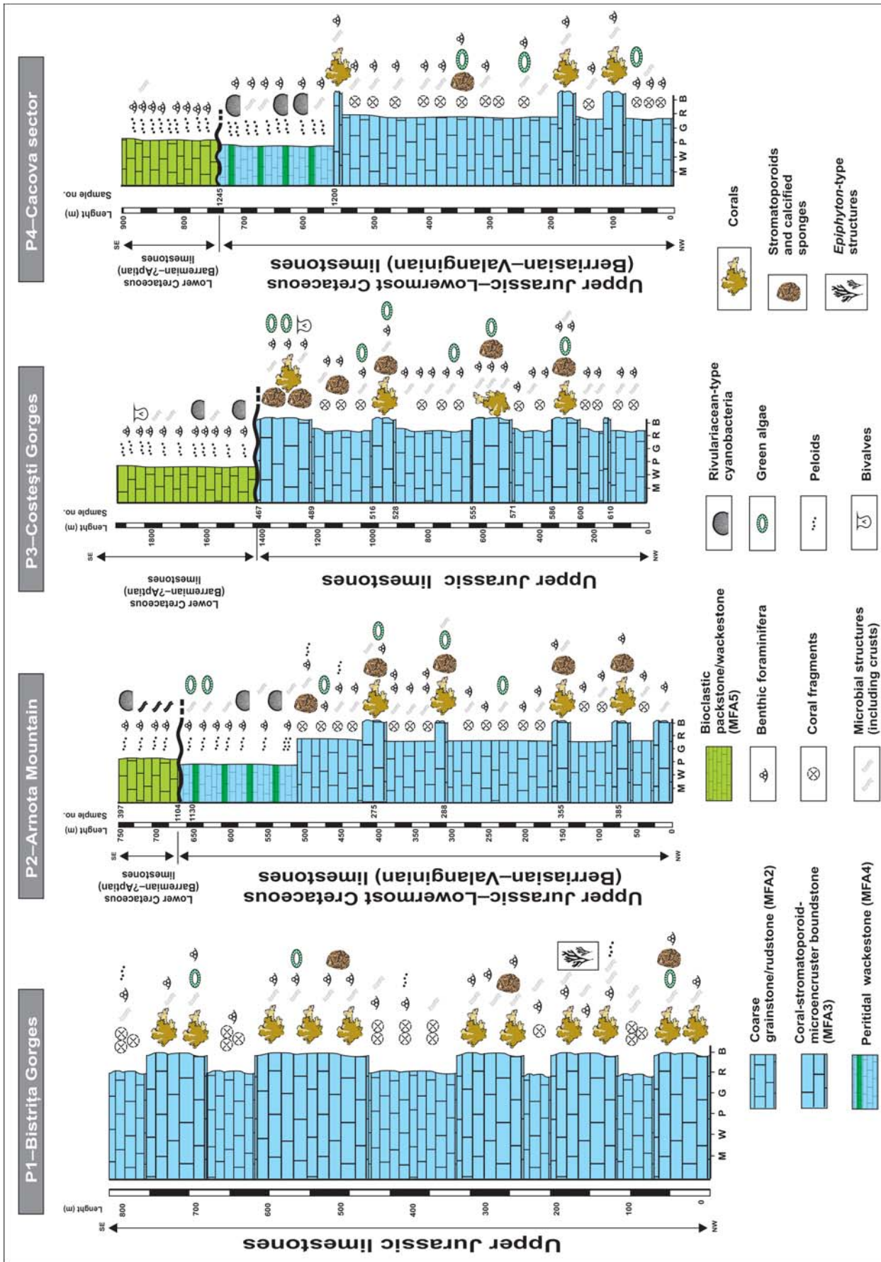
Fig. 3. General succession of the limestone deposits of the Buila-Vânturarița Massif (sections P1 to P4).
