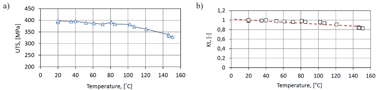
Fig. 12. Ultimate tensile strength (UTS) at different temperatures (a) and relative tensile strength K_t (b)
