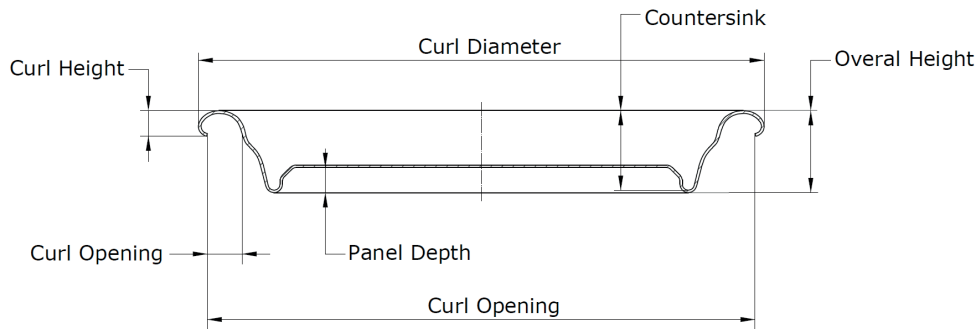
Fig. 16. Nomenclature of the geometric parameters dimensions for beverage can end
