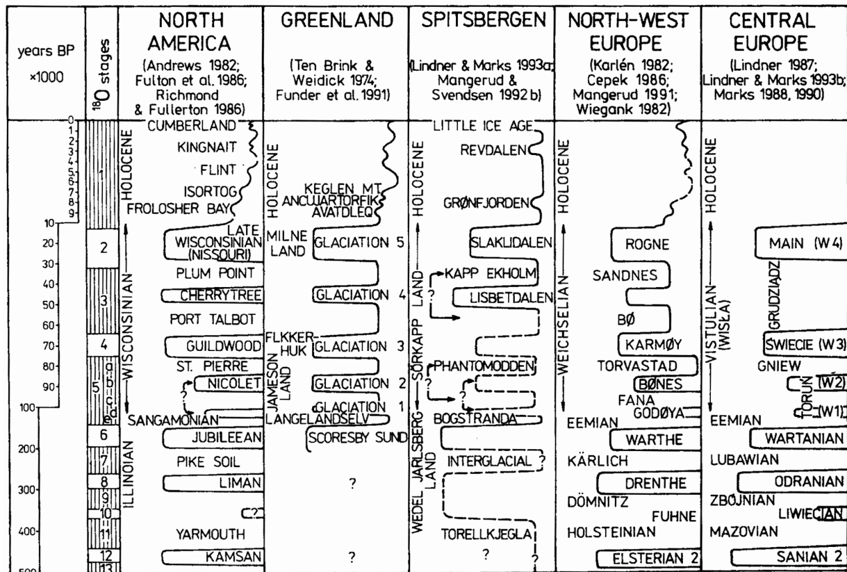
Fig. 16. Correlation of Quaternary stratigraphic schemes for Northern America, Greenland, Spitsbergen and Europe (Lindner, Marks 1993)
