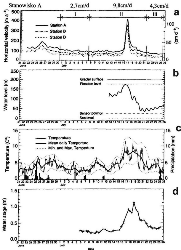
Fig. 23. Dynamics of Hansbreen movements during summer 1999 (Vieli et al. 2003) a – horizontal velocity, I-III – periods of ablation, b – pressure in ice aven as a water level, c – air temperature and precipitation at Polish Polar Station, d – water level in glacial river of Werenskioldbreen
