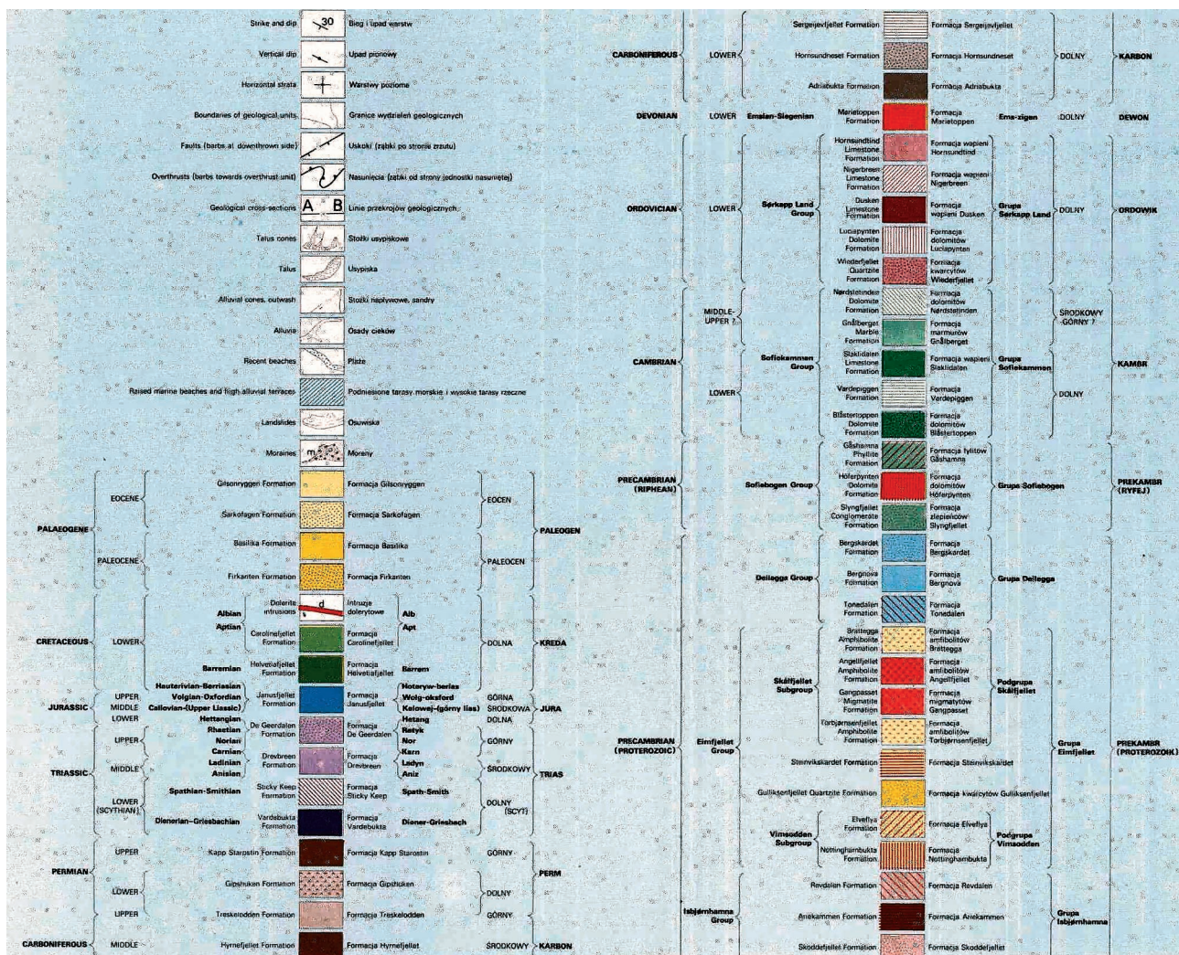
Fig. 9. Geological map of the northern part of Hornsund (Birkenmajer 1990)
