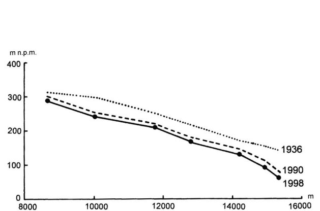
Fig. 25. Changes in thickness of Hansbreen along the ablation zone (Jania 2004)
