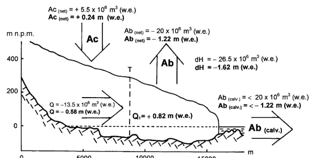
Fig. 29. Mass balance for Hansbreen along longitudinal profile of glacier (Jania 2004) – average values of water equivalent (w.e.) for 1990–1998 Ac – accumulation netto, Ab – ablation netto, Ab (calv.) – ablation by calving, Q_T – flow of ice below ELA, dH – decrease in glacier thickness.
