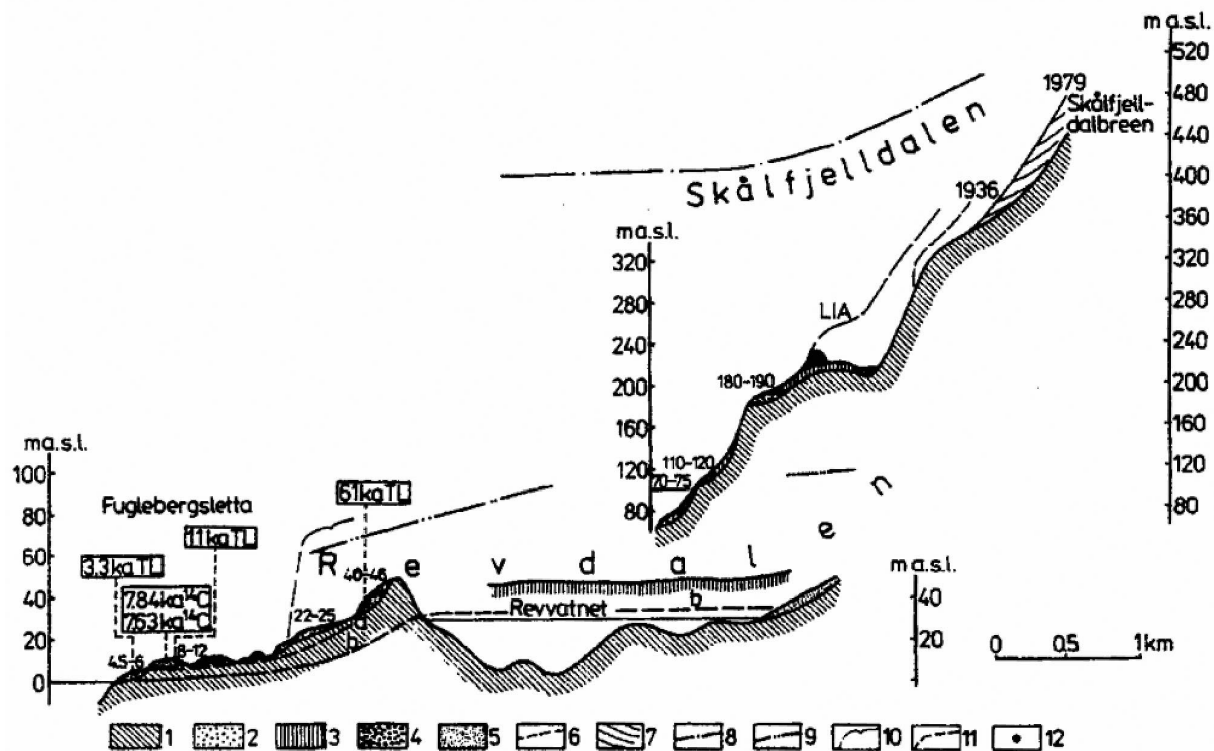
Fig. 17. Schematic geological cross-section through Revdalen and Fuglebergsletta (Lindner et al. 1984, corrected) 1 – bedrock, 2 – marine gravels (altitude of marine terraces in m a.s.l.), 3 – till, 4 – deposits of ice-moraine ridges, 5 – sand and gravel of outwash-plains, 6 – older (a) and younger (b) outwash-plain, 7 – glacier ice, 8 – old glacier fronts, 9 – young glacier fronts, 10 – the biggest range of glaciers in Holocene, 11 – range of glaciers during LIA (Little Ice Age), 12 – sampling sites for dating
