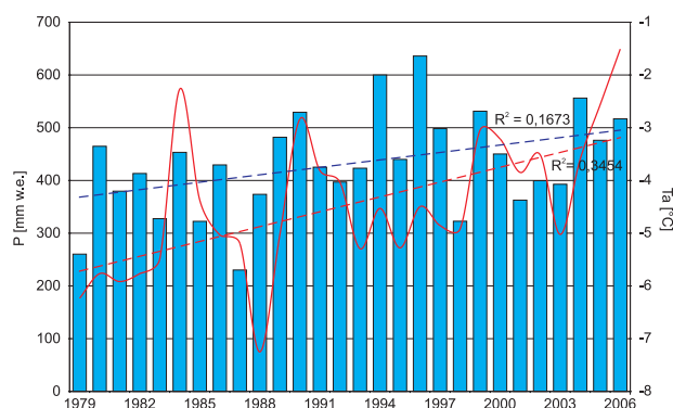
Fig. 4. Course of annual precipitation (P) and air temperature (Ta) in Polish Polar Station at Hornsund
