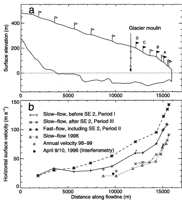
Fig. 28. Velocity of ice surface for Hansbreen (Vieli et al. 2003) a – sampling sites in glacial avens, b – surface velocity of ice.
