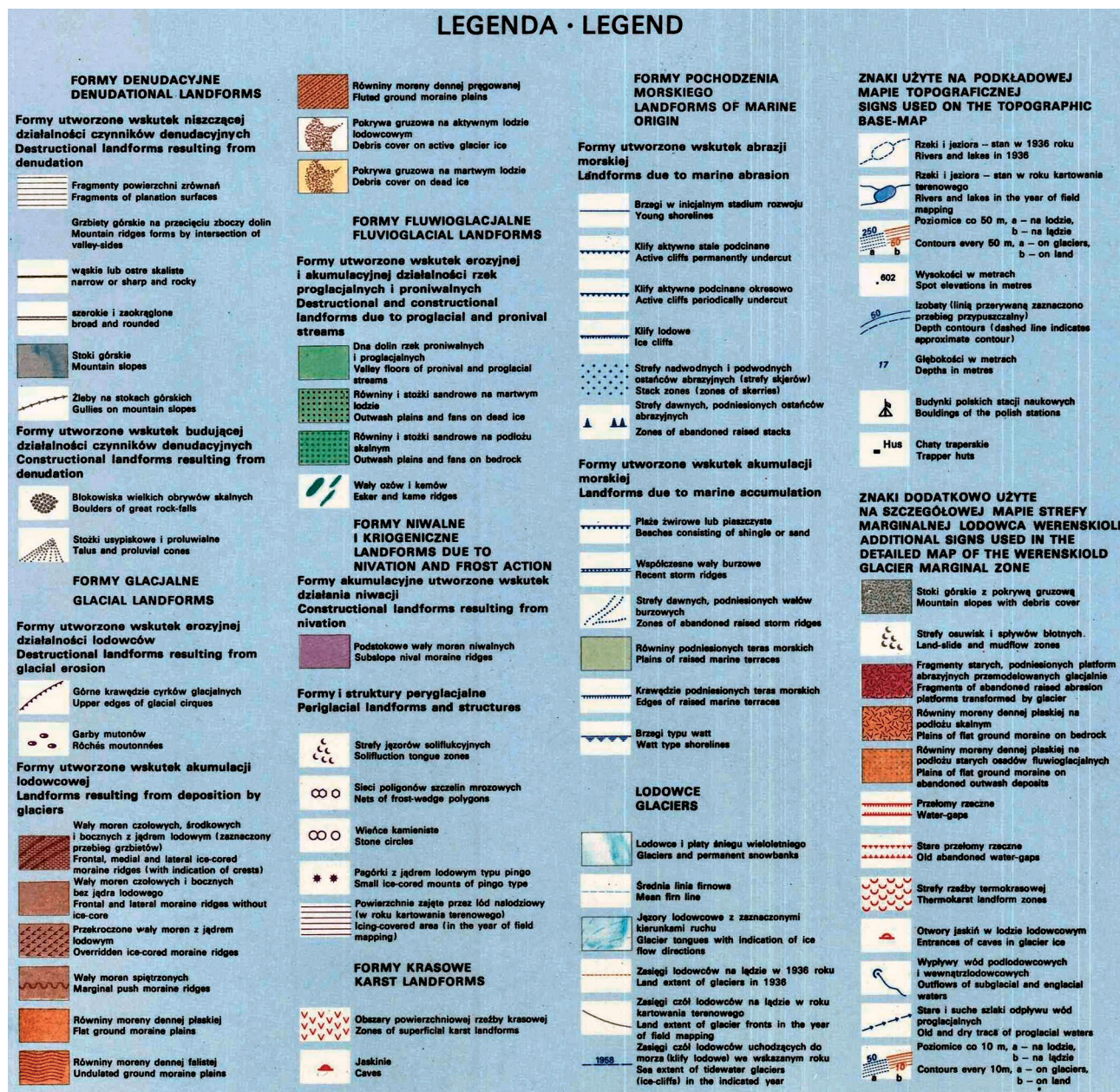
Fig. 10. Geomorphological map of the northern part of Hornsund (Karczewski 1984)
