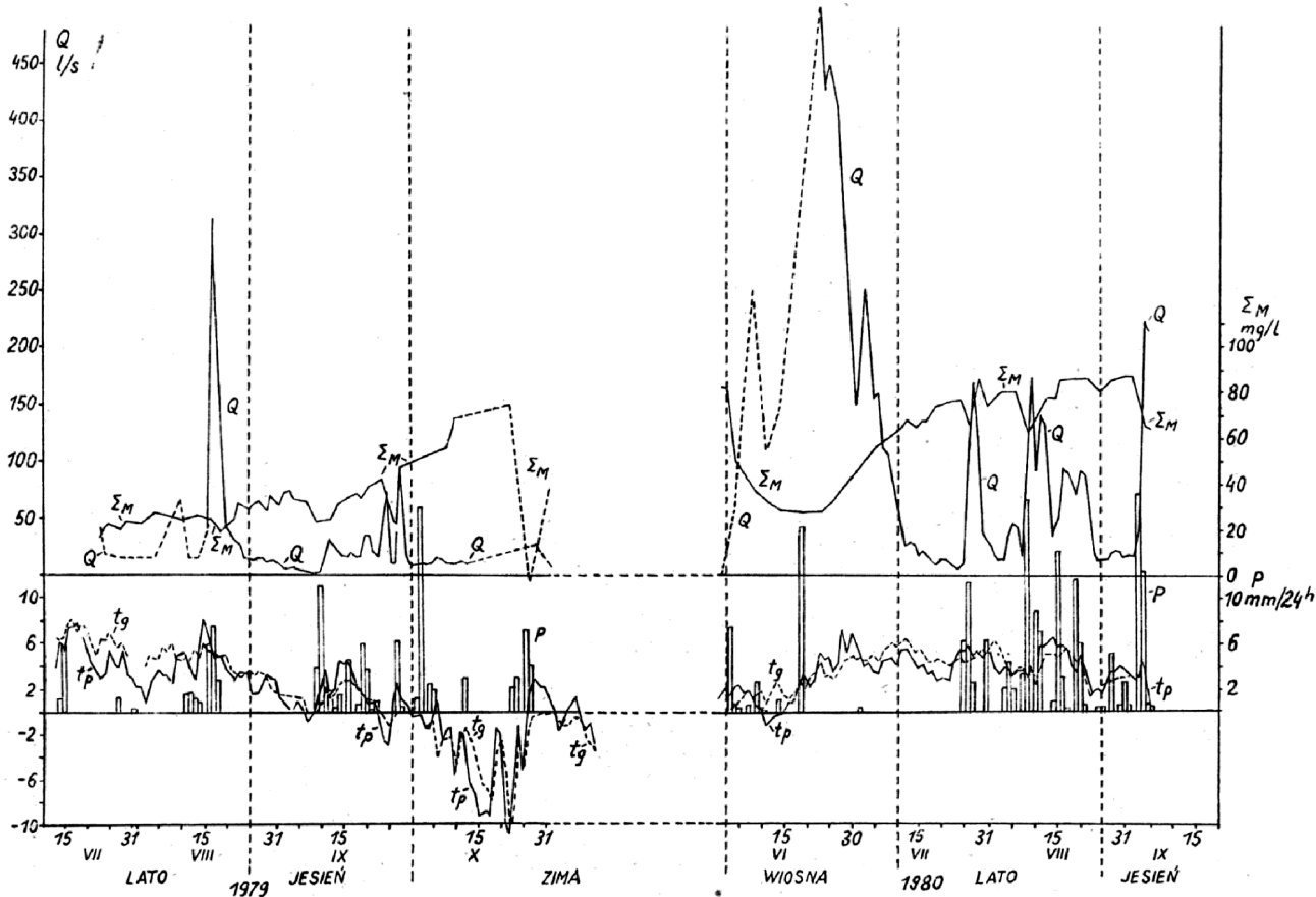
Fig. 19. Course of discharge (Q) in the background of physicochemical properties of stream water and meteorological elements within the Fuglebekken catchment during hydrological year 1979/80 (Pulina 1986) tg – ground temperature at depth 5 cm, \Sigma M – total mineralization of stream water, P – precipitation, tp – air temperature.
