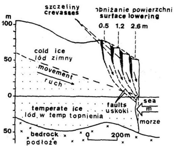
Fig. 24. Cross-section of glacier front, Hansbreen (Jania 1988) Cross-section shows mechanism of calving in the form of glacial slips; m – subwater melting.
