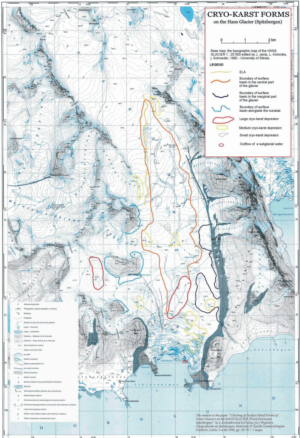
Fig. 30. Distribution of cryo-karst forms on the Hansbreen (Kolondra, Pulina 1998)
