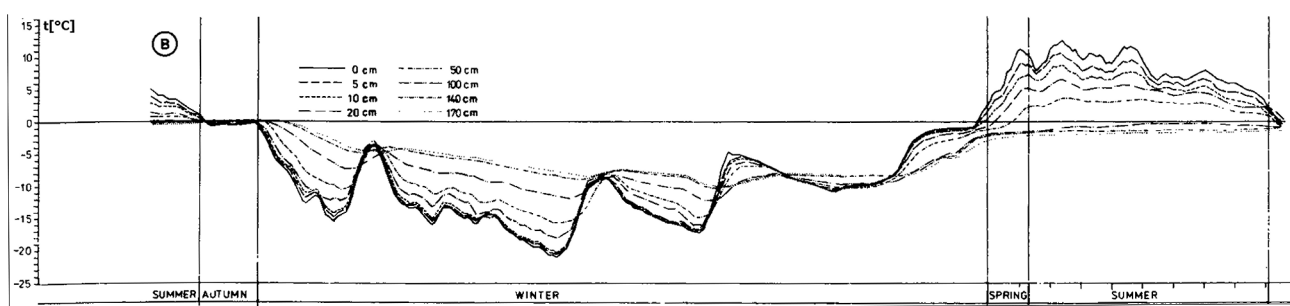
Fig. 20. Annual (1985/86) course of ground temperature at different depth in Fuglebekken catchment (Głowacki et al. 1990)
