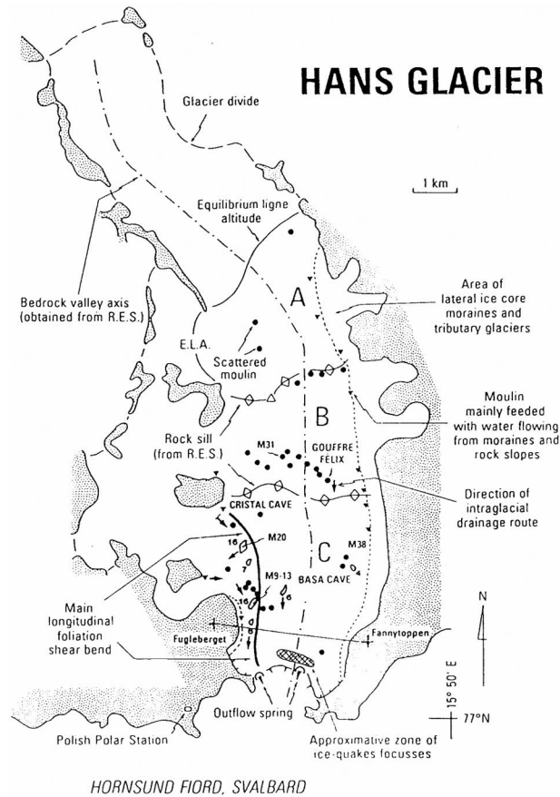
Fig. 13. Location of ice caves in Hansbreen (Schroeder 1995)
