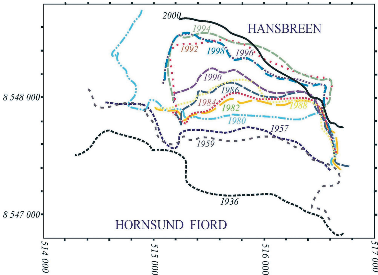
Fig. 27. Changes in front location for Hansbreen (Kolondra 1993)
