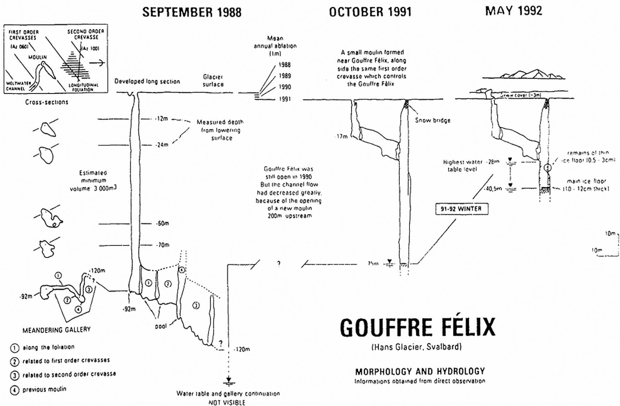
Fig. 14. Gouffre Félix in Hansbreen (Schroeder 1995)
