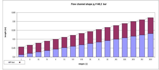
Fig. 17. IP flow channel shape for a division pressure ratio of 0,6
