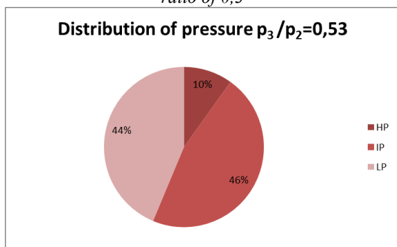
Fig. 8. Percentage distribution of enthalpy reduction at individual parts of cylinders for a division pressure ratio of 0,53
