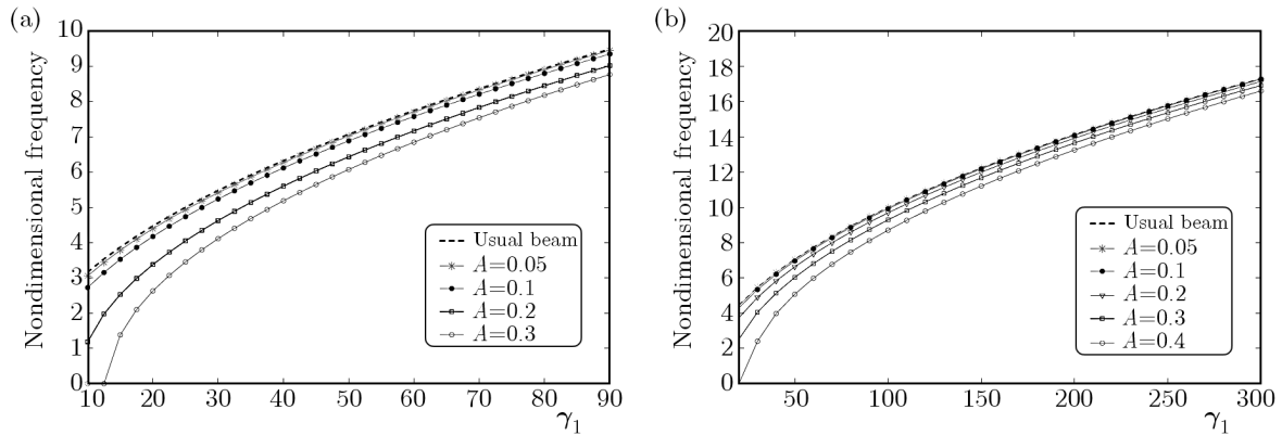
Fig. 5. Comparison of fundamental frequencies of the usual beam and quintic nonlinear beam as a function of \gamma_1 , (a) S-S beam, (b) C-C beam
