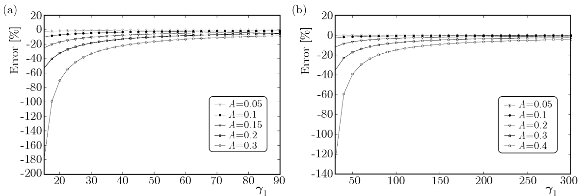
Fig. 6. The percent of error in approximating the natural frequency of the usual beam as a function of \gamma_1 , (a) S-S beam, (b) C-C beam
