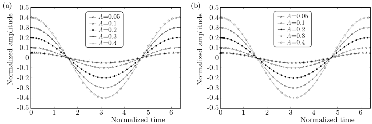
Fig. 2. Comparison between analytical and numerical results for different initial amplitudes, symbols: numerical solution, solid line: analytical solutions, (a) S-S beam, (b) C-C beam
