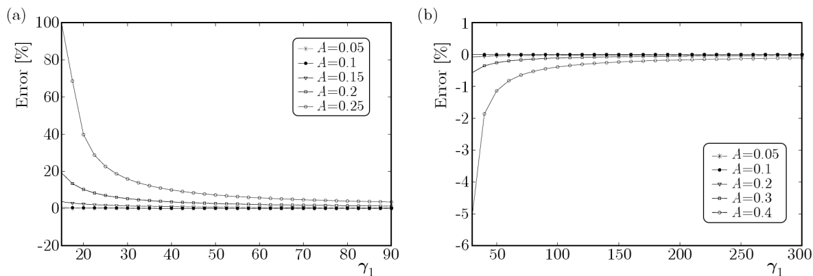
Fig. 7. The percent of error in approximating the natural frequency of the cubic nonlinear beam as a function of \gamma_1 , (a) S-S beam, (b) C-C beam
