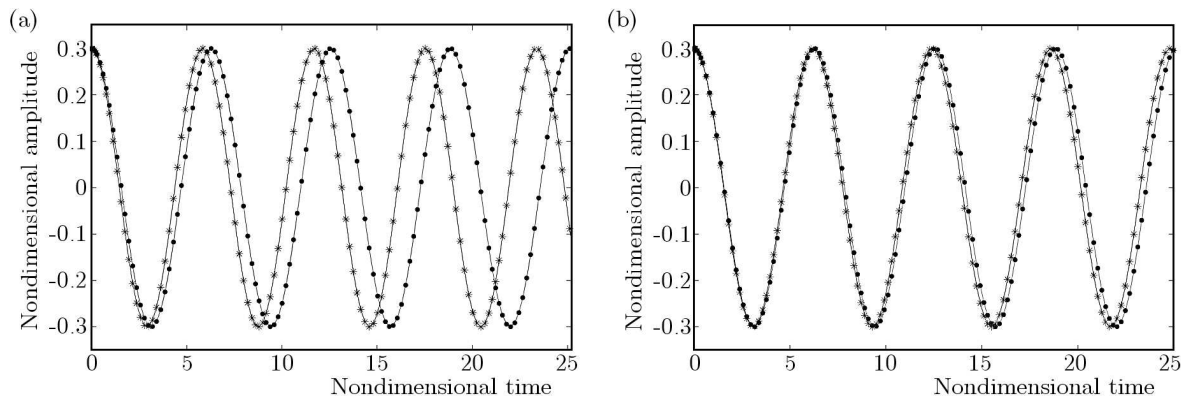
Fig. 3. The impact of nonlinear terms on dynamical behavior of the beam for A = 0.3 , -* – usual beam theory, - \bullet - – quintic nonlinear beam, (a) S-S beam, (b) C-C beam
