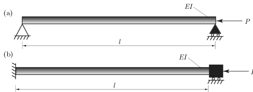
Fig. 1. Configuration of a uniform Euler-Bernoulli beam (a) simply supported beam, (b) clamped-clamped beam
