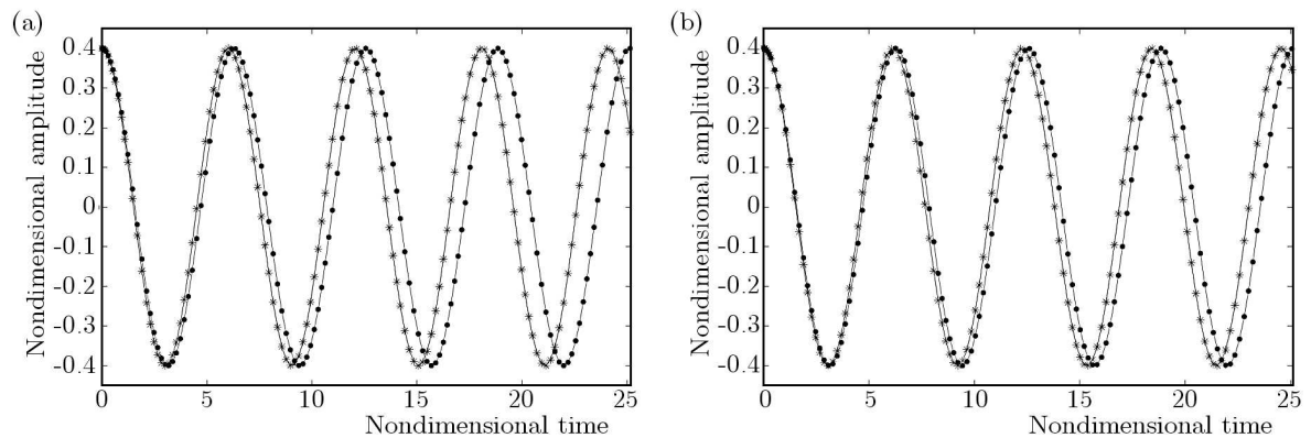
Fig. 4. The impact of nonlinear terms on dynamical behavior of the beam for A = 0.4 , -* – usual beam theory, - \bullet - – quintic nonlinear beam, (a) S-S beam, (b) C-C beam
