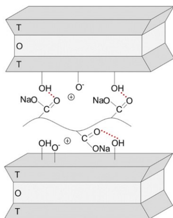
Fig. 4. Hydrogen bonds in the MMT- co -MA/AA hybrid system
