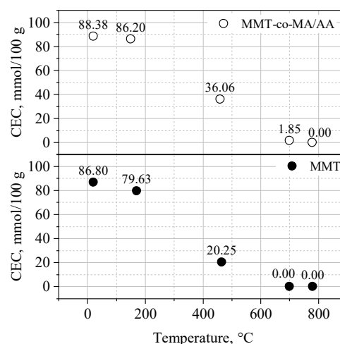
Fig. 7. The ion exchange capacity obtained for samples MMT and MMT- co -MA/AA
