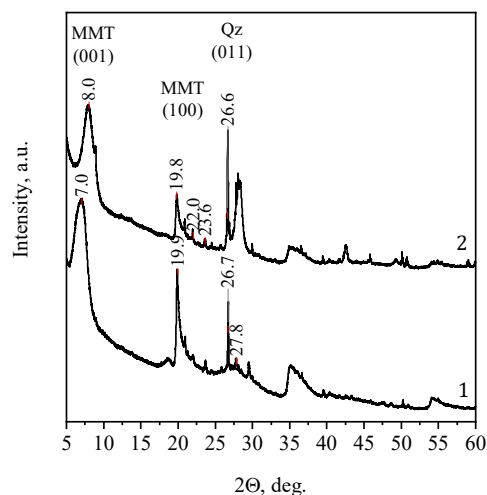
Fig. 2. XRD diffractograms of 1) MMT, 2) MMT- co -MA/AA
