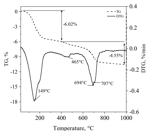
Fig. 6. TG–DTG curves of MMT (a), MMT- co -MA/AA (b)
