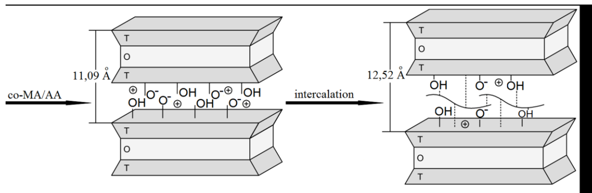
Fig. 5. Synthesis route of co -MA/AA intercalated MMT hybrid
