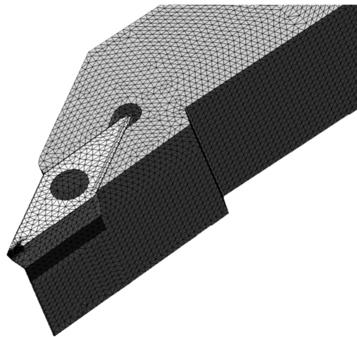
Fig. 3. Mounted tool with FEM mesh (SolidWorks)
