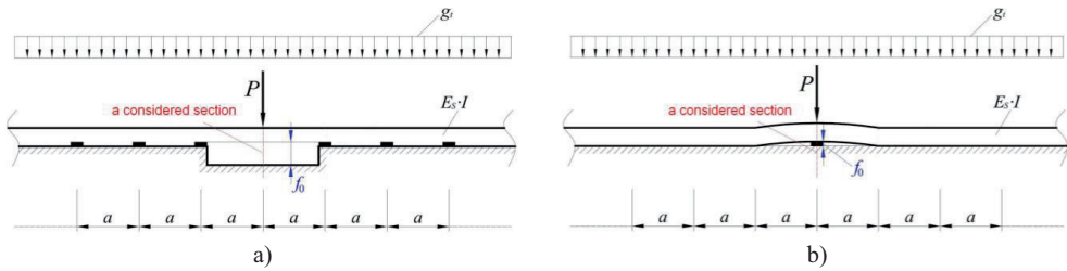
Fig. 2. The schemes of local imperfections generated in railway track
