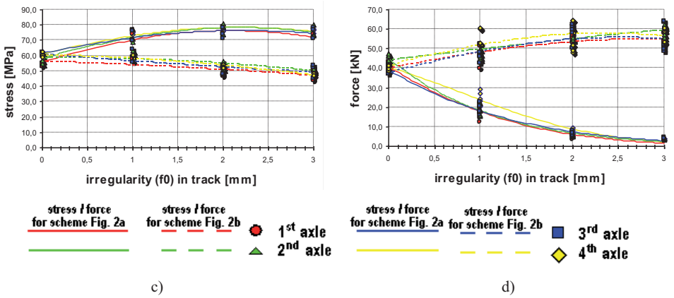
Fig. 4. An obtained values due to induced an author's irregularity in the railway track (for successively locomotive's axles)
