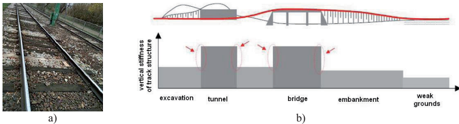
Fig. 1. Examples of arising imperfections in railway track [4,11,12,13]
