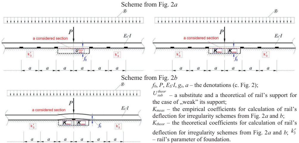
Fig. 5 The exemplary assumed simplified schemes for a analysis of generated irregularities in the track a) a decreasing of a considered section in track; b) a raising of a considered section in track
