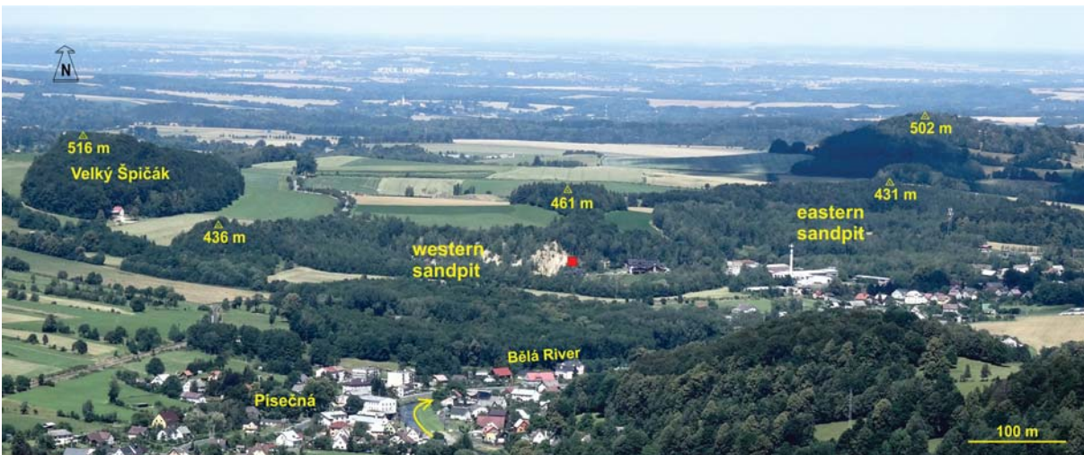
Text-fig. 4. View of the study area from the north-western slope of the Zlaté Hory Highlands. Red rectangle represents the section shown in detail in Text-figs 7 and 8
