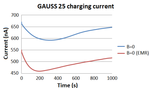
Fig. 5. The graphic dependence of the charging current on the time, the sample GAUSS 25 before the influence of EMR and after the influence of EMR
