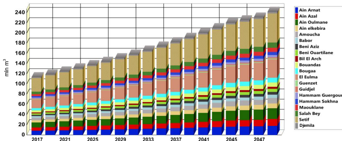
Fig. 5. Evolution of water demand in Setif Province – reference scenario; source: own study
