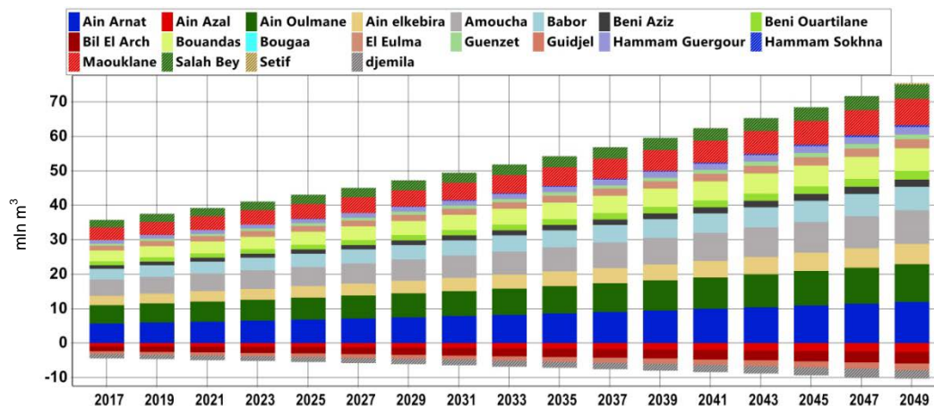
Fig. 8. Evolution of unmet water demand for scenario demand management and lifestyle development (DMLD) relative to a reference; source: own study
