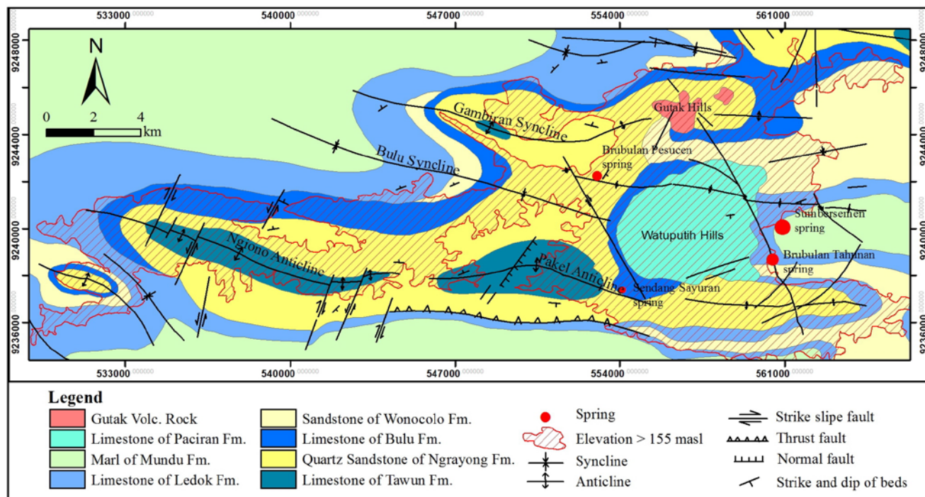
Fig. 14. The zone above 155 m a.s.l. showing the diverse rock formations and geological structures of the study area based on a 1:100,000 geological map; source: own elaboration
