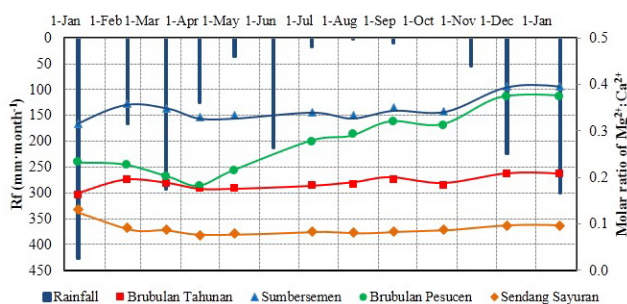
Fig. 11. Monthly rainfall and Mg^{2+}:Ca^{2+} ratio variations at four major springs in the study area; source: own study
