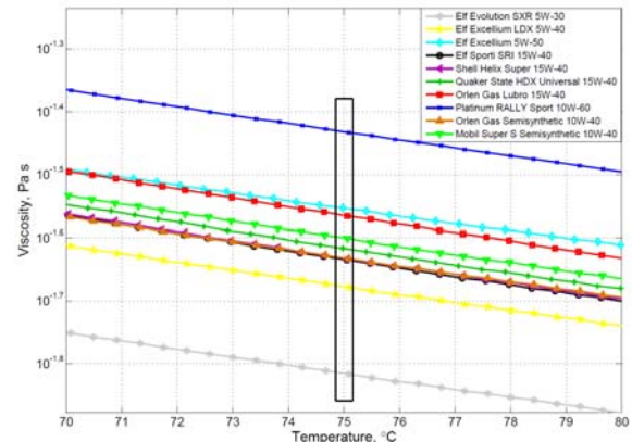
Fig.6. The characteristics of viscosity of engine oils in the referential temperature.
