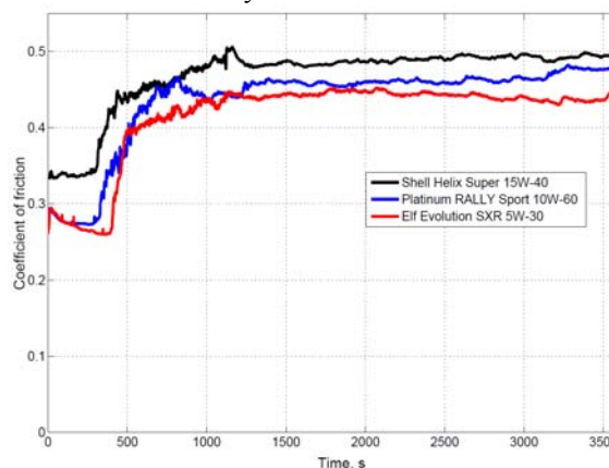
Fig. 4. Exemplary chart of coefficients of friction for mineral, semisynthetic and synthetic oils.
