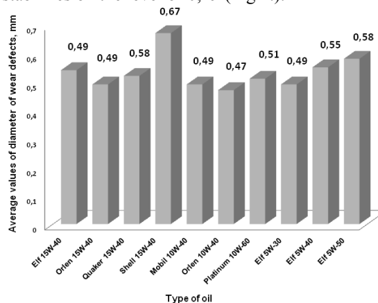
Fig. 3. Specification of wear defects of engine oils tested by ASTM D2266-01
