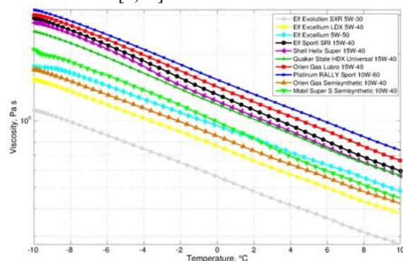
Fig. 5. The characteristics of viscosity of engine oils in the range of sub-zero and low temperatures
