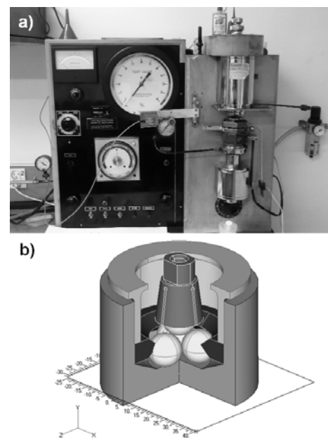
Fig.1. Four-ball testing machine by Roxana: a) main view, b) friction node
