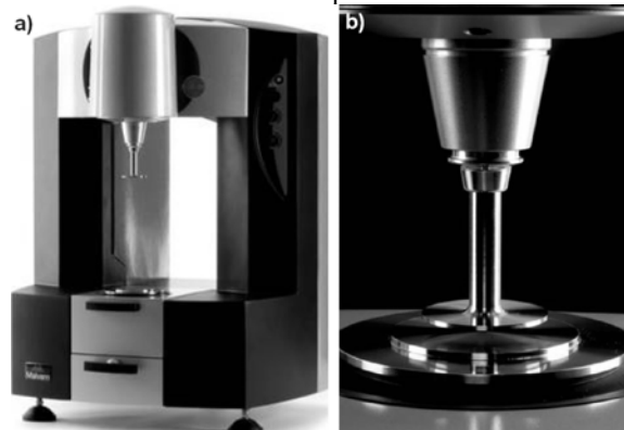
Fig. 2. Rotational rheometer Kinexus Pro: a) main view, b) testing node
