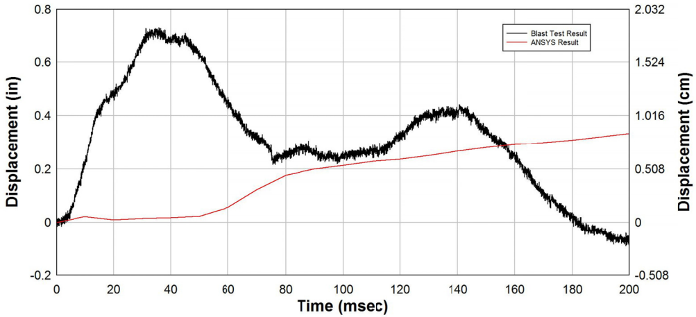
Fig. 6. Deflection Comparison of Left-Center Vertical Steel Member
