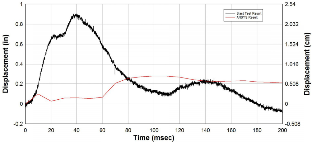
Fig. 7. Deflection Comparison of Far-Left Vertical Steel Member
