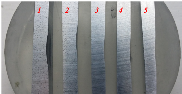
Fig. 1. Cross-sections of specimens 1 to 5 after wear test
