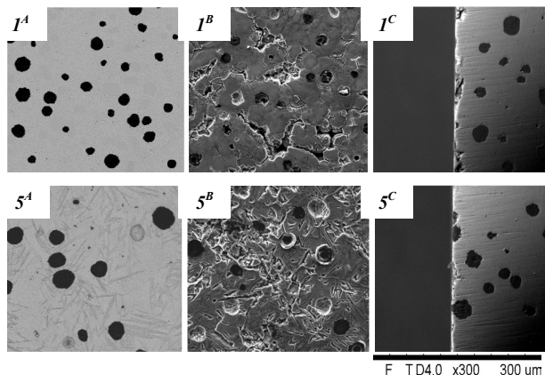
Fig. 3. SEM images of the alloys No. 1 and No. 5: surfaces before corrosion tests, made by BSE technique ( I^A , 5^A ); surfaces after potentiodynamic tests for 168 hours of exposure, made by SE technique ( I^B , 5^B ) and cross-sections after potentiodynamic tests for 168 hours of exposure, made by SE technique ( I^C , 5^C )
