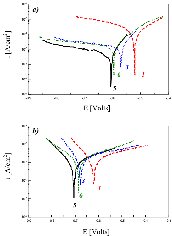
Fig. 2. Polarisation curves of the alloys No. 1, 3, 5 and 6 after: a) 1 hour, b) 168 hours of exposure in 3% aqueous NaCl solution
