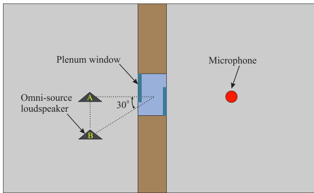
Fig. 2. Schematic diagram of the experimental set-up for experiments A and B.
