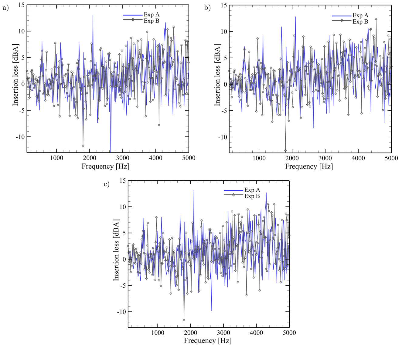
Fig. 5. IL_2 obtained by the plenum window with HRs (attached 45^\circ jagged flap) when comparing with the case of without resonators for experiments A and B: a) white noise, b) traffic noise, c) construction noise.
