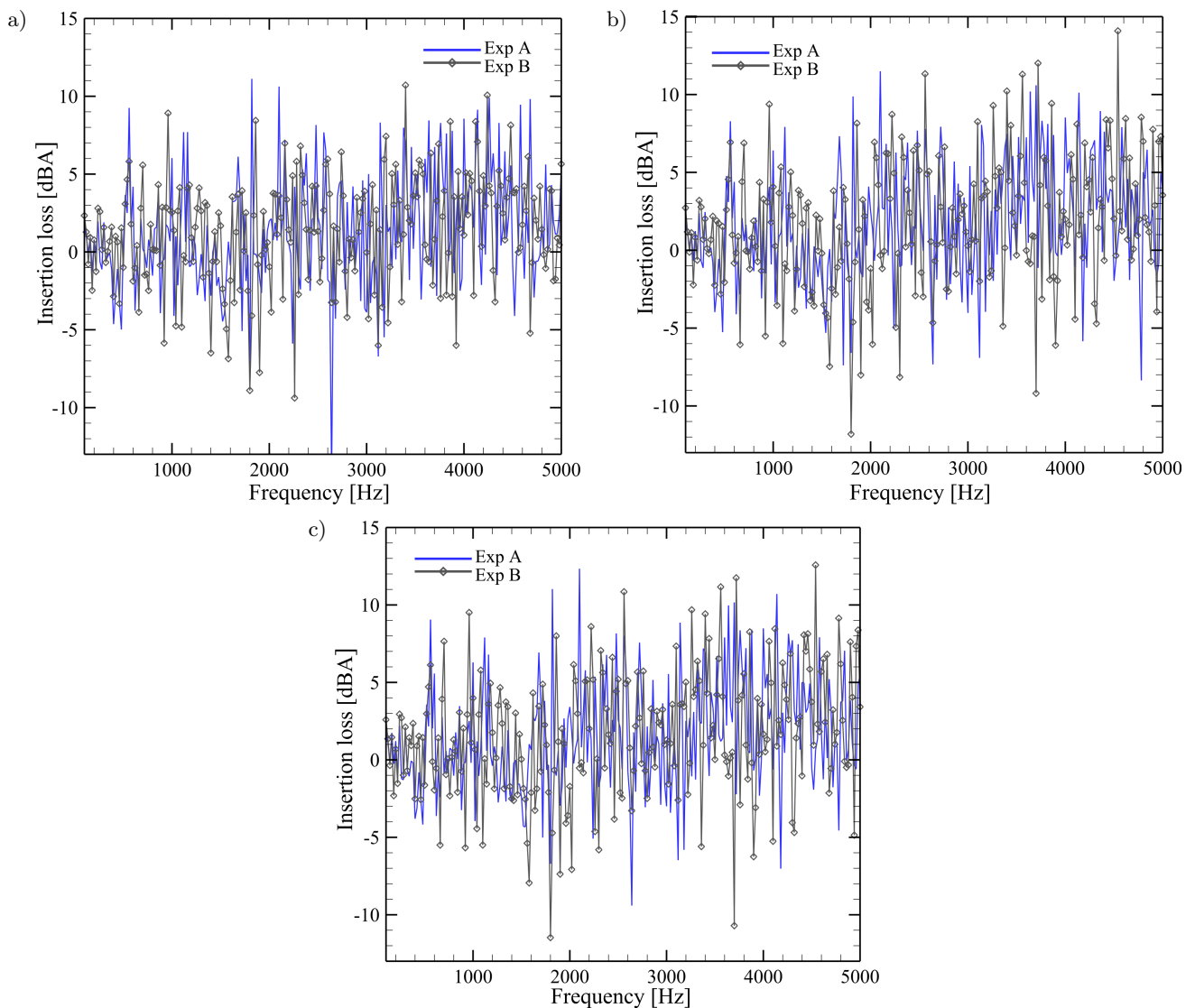
Fig. 4. IL_2 obtained by the plenum window with HRs (attached 90° jagged flap) when comparing with the case of without resonators for experiments A and B: a) white noise, b) traffic noise, c) construction noise.
