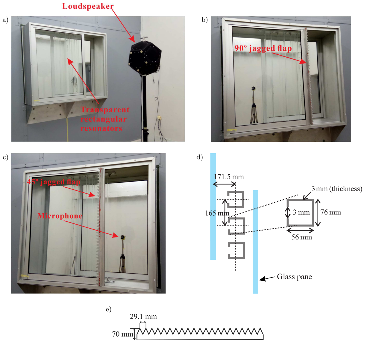
Fig. 1. a) Experimental set-up of the plenum window with rectangular HRs at reverberation room, b) plenum window with attached 90° jagged flap, c) plenum window with attached 45° jagged flap, d) geometry of the plenum window with HRs (top view), e) geometry of the jagged flap.
