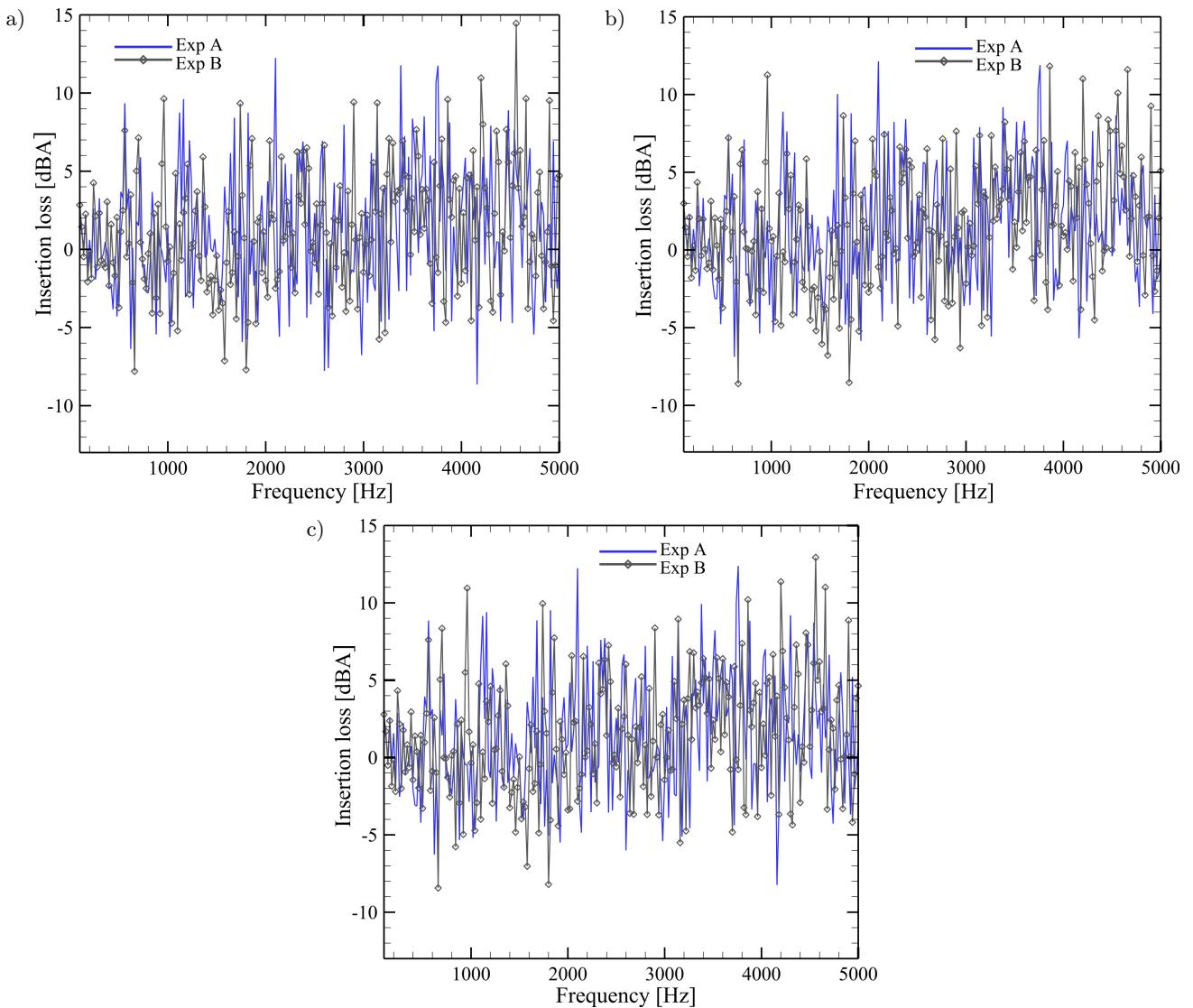
Fig. 3. IL_2 obtained by the plenum window with HRs (without jagged flap) when comparing with the case of without resonators for experiments A and B: a) white noise, b) traffic noise, c) construction noise (the data are recorded at interval of 2 Hz, but the results are presented at interval of 20 Hz for clearer presentation of the IL trends).
