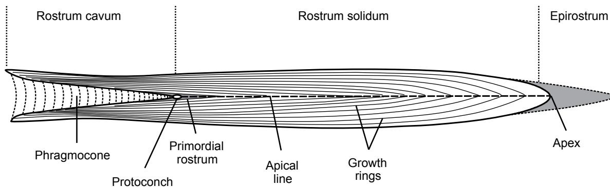
Fig. 1. Morphology and internal structure of the schematized belemnite rostrum
