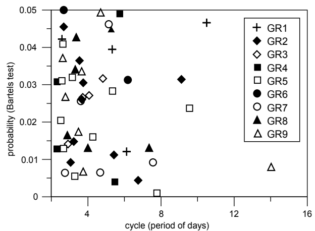
Fig. 8. Relationship between belemnite growth cycles and their probability (Bartels test values). The cycles were determined using a Cycles Analysis and Time Series Software (CATS) version 1.0
