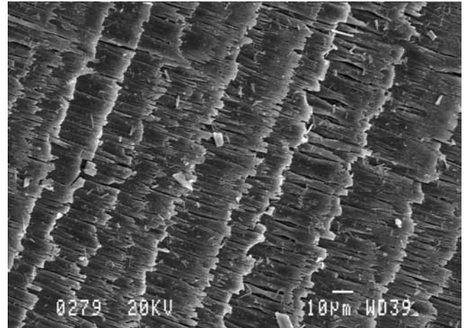
Fig. 4. Clearly visible growth rings on the etched surface of a belemnite rostrum. The rings form distinct belt morphology. Sample no. GR5 ( Hibolites jurensis ). SEM image
