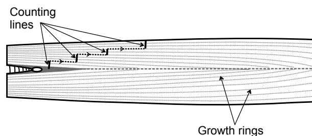
Fig. 3. Schematized diagram showing the counting method of growth rings on the etched thick section of belemnite rostrum
