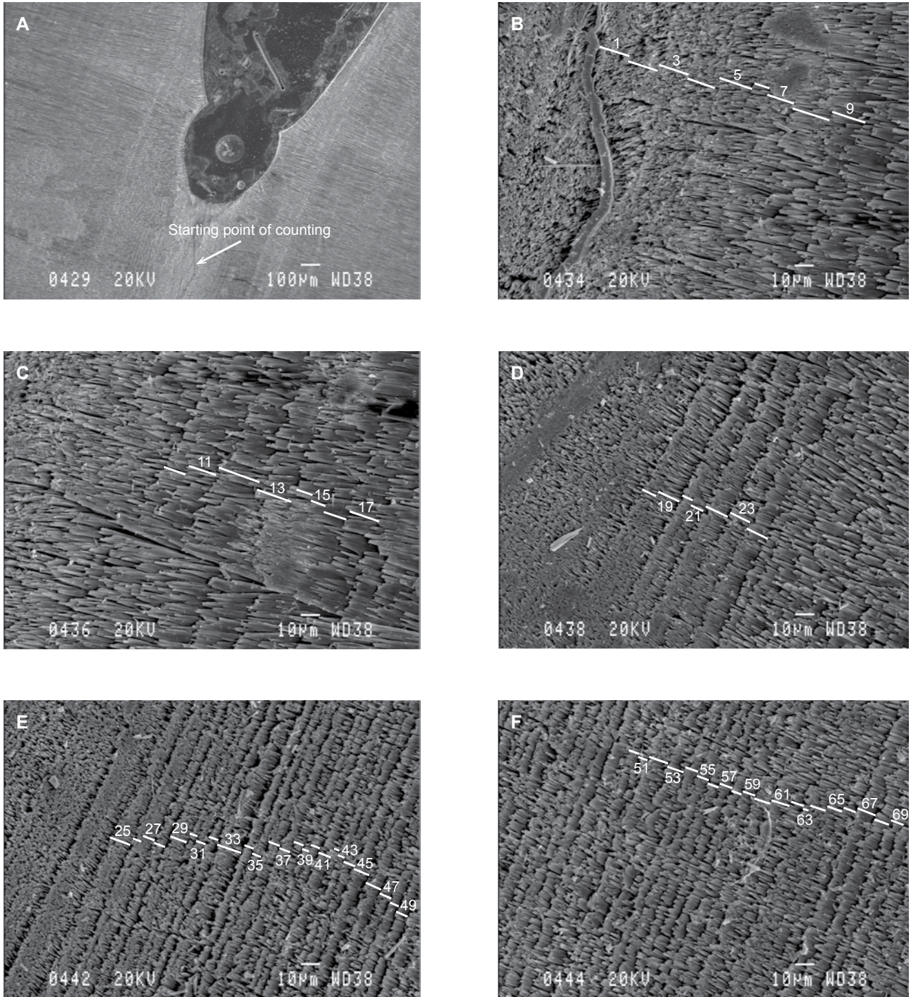
Fig. 6. A-X. Continuous record of all (two hundred sixty one) growth rings of the rostrum GR8
