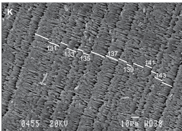
( Pachybelemnopsis fusiformis ). Successive growth rings are numbered. SEM images
