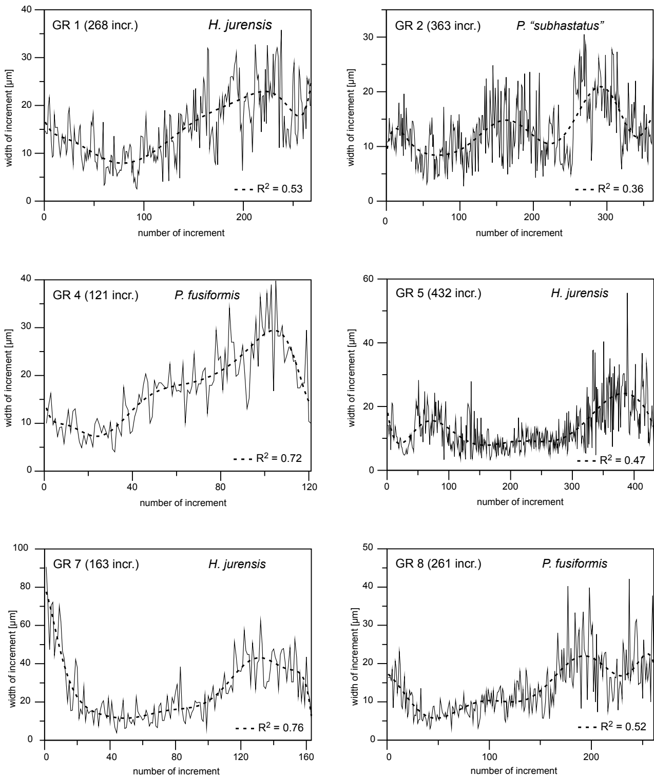
Fig. 7. Relationship between the number of belemnite growth increments and their width. Tenth degree polynomial functions Coefficients of determination of the functions ( R^2 ) are shown in the bottom
