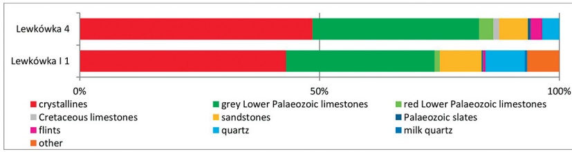
Fig. 10. Percentages of the various petrographical groups of the Warthian fluvioglacial fresh gravel (4–10 mm fraction) in zone IV (Piotrków Plain) (for legend see Table 2)
