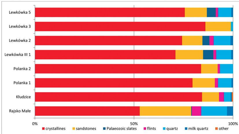
Fig. 11. Percentages of the various petrographical groups of the Warthian fluvioglacial weathered gravel (4–10 mm fraction) in zone IV (Piotrków Plain) (for legend see Table 2)
