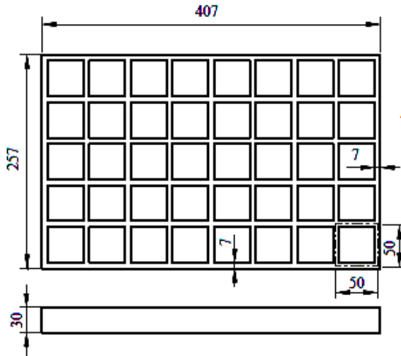
Fig. 1. The geometry of the initial grate adopted for research
