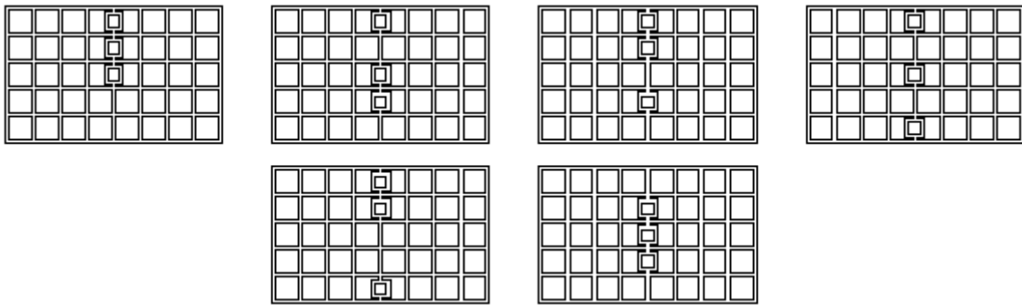
Fig. 5. Structures of grates comprising 3 flexible segments in lengthwise orientation
