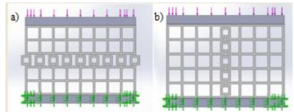
Fig. 3. Grates containing maximum number of flexible segments in orientations: crosswise (a) and lengthwise (b) [4]
