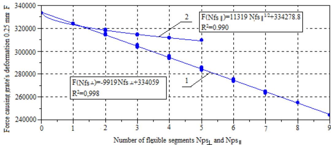
Fig. 6. The results of measurements and calculations for grates with flexible segments in orientation crosswise (1) and lengthwise (2)
