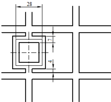
Fig. 2. The shape and dimensions of the flexible segment
