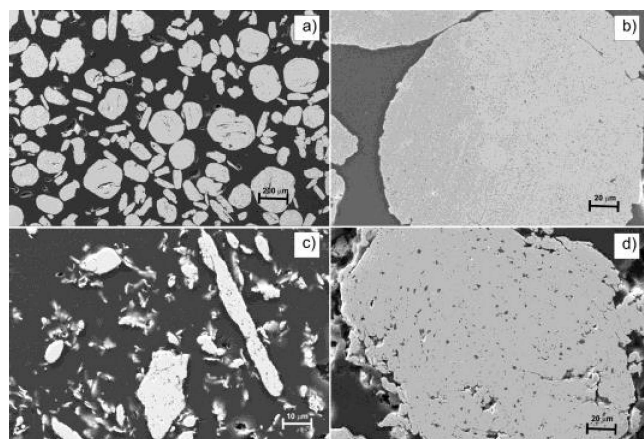
Fig. 5. Flake microstructure resulting from mechanical synthesis of powder mixtures (200 rpm): a-b) Cu_{spher} - 5\%ED Al_2O_3 and c-d) Cu_{dend} - 5\%ED Al_2O_3
