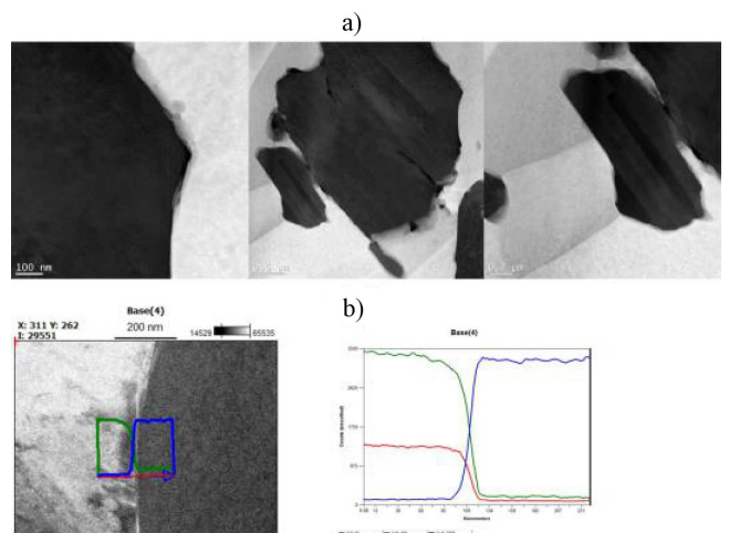
Fig. 10. a) TEM images, and b) linear distribution of elements (Cu, Al, O) across the metal-ceramic interface of the \text{Cu}_{\text{dendritic}} - \text{ED Al}_2\text{O}_3 composite (200 rpm)
