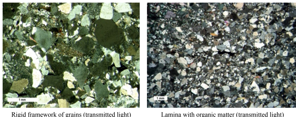
Fig. 1. Photomicrographs (transmitted light) of a sample of fine-grained quartz sandstone, medium sorted, of porous and contact clay cementation
