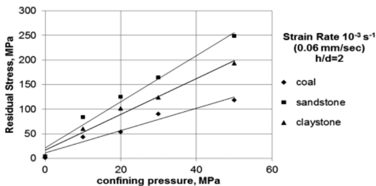
Fig. 9. Dependence of residual stress in sedimentary rocks of the USCB on the confining pressure
