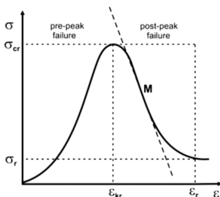
Fig. 6. Determining post-critical modulus M , residual stress ( \sigma_r ), and residual strain ( \epsilon_r ) based on the shape of the stress-strain curve
