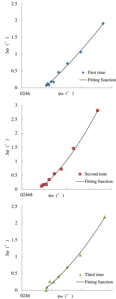
Fig. 10. Extinction curves
