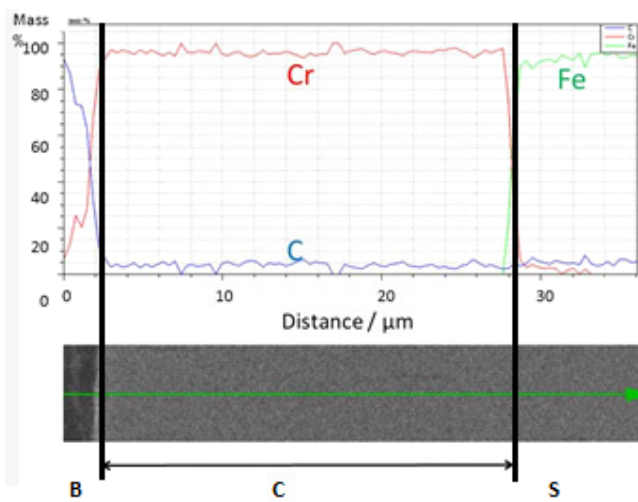
B - Bakelite, C - Coating, S - Steel
