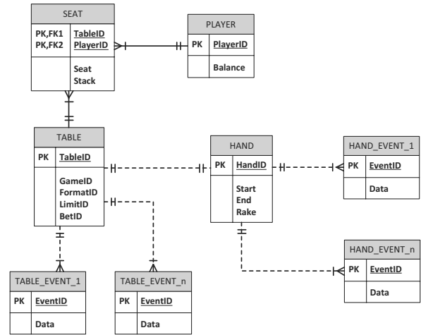
Fig. 1. High level conceptual data model of a poker hand.
