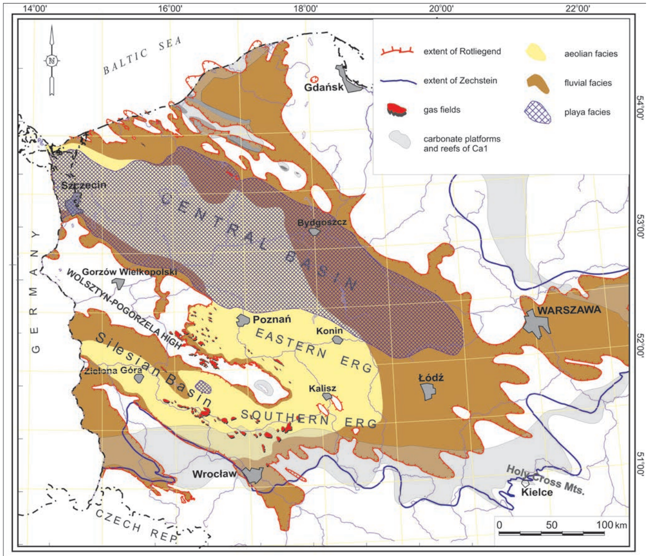
Fig. 6. Location map of Rotliegend reservoirs and Zechstein Limestone (Ca1) in the light of reservoir facies distribution (modified after Papiernik et al. , 2008)
