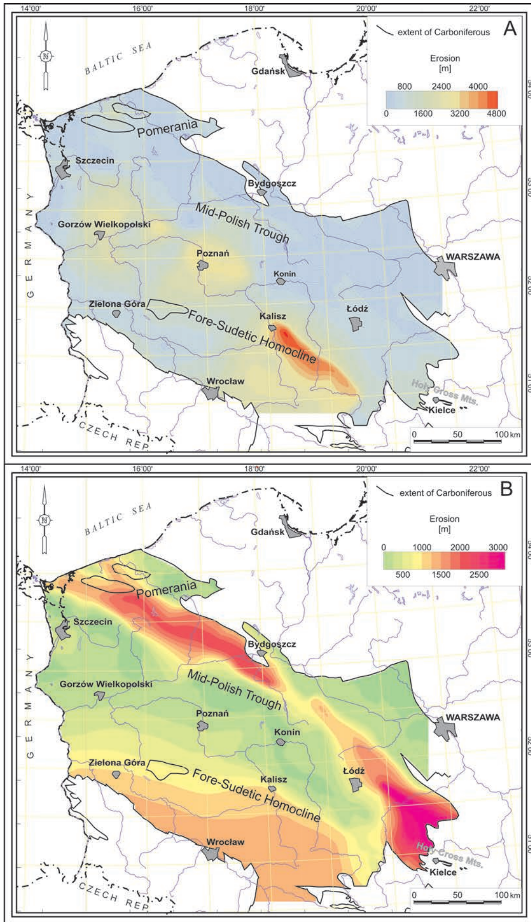
Fig. 9. Calculated erosion: post-Variscan (A), Laramide (B)
