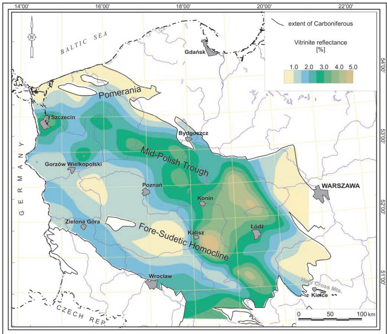
Fig. 11. Calculated present-day vitrinite reflectance at top of Carboniferous
