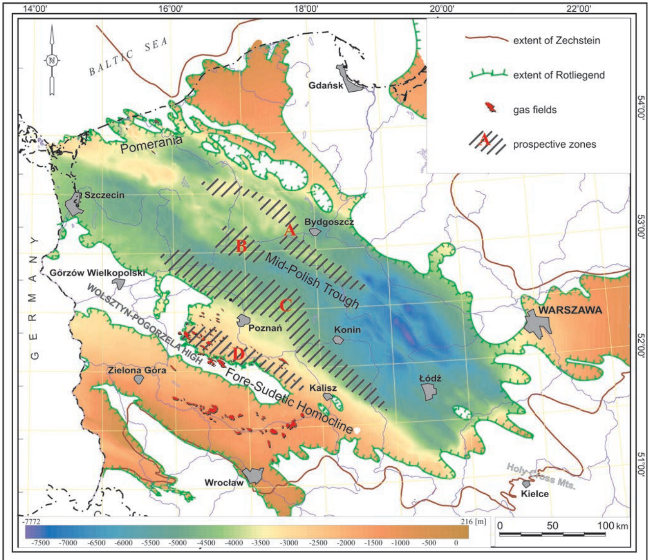
Fig. 16. Location map of prospective zones at top of Rotliegend (modified after Burzewski et al. , 2009; Górecki et al. , 2011)
