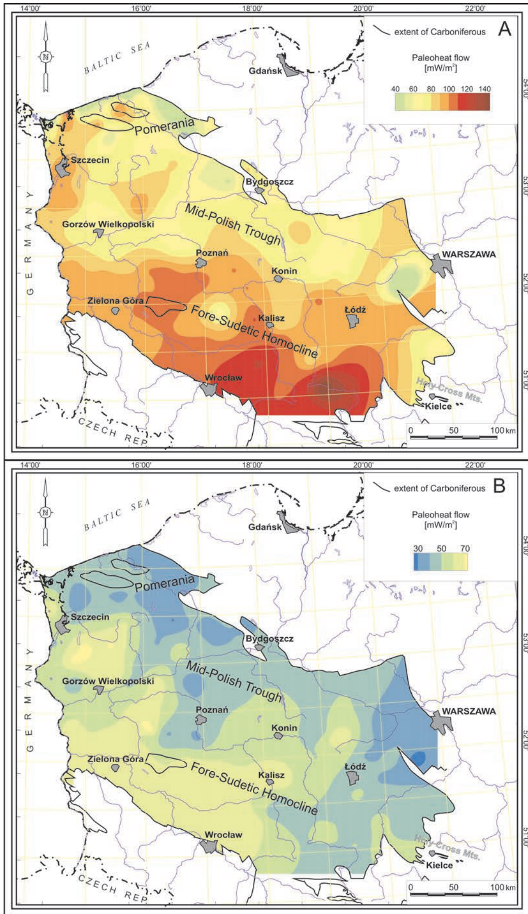
Fig. 10. Palaeo-heat flow: Variscan (A), Cretaceous (B)
