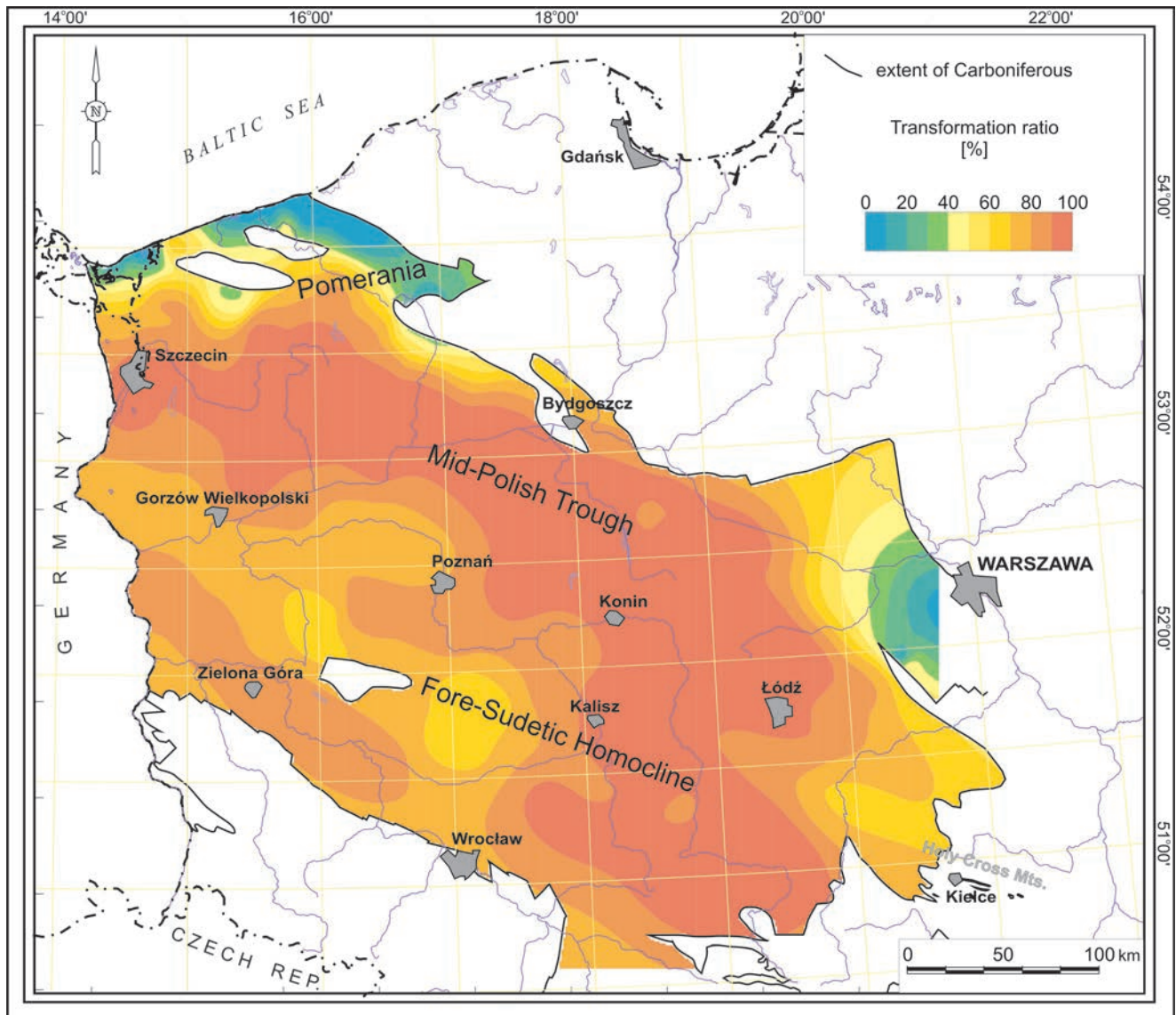
Fig. 14. Degree of kerogen transformation (TR%) in Carboniferous source rocks (referred to top of Carboniferous) calculated for the end of Cretaceous
