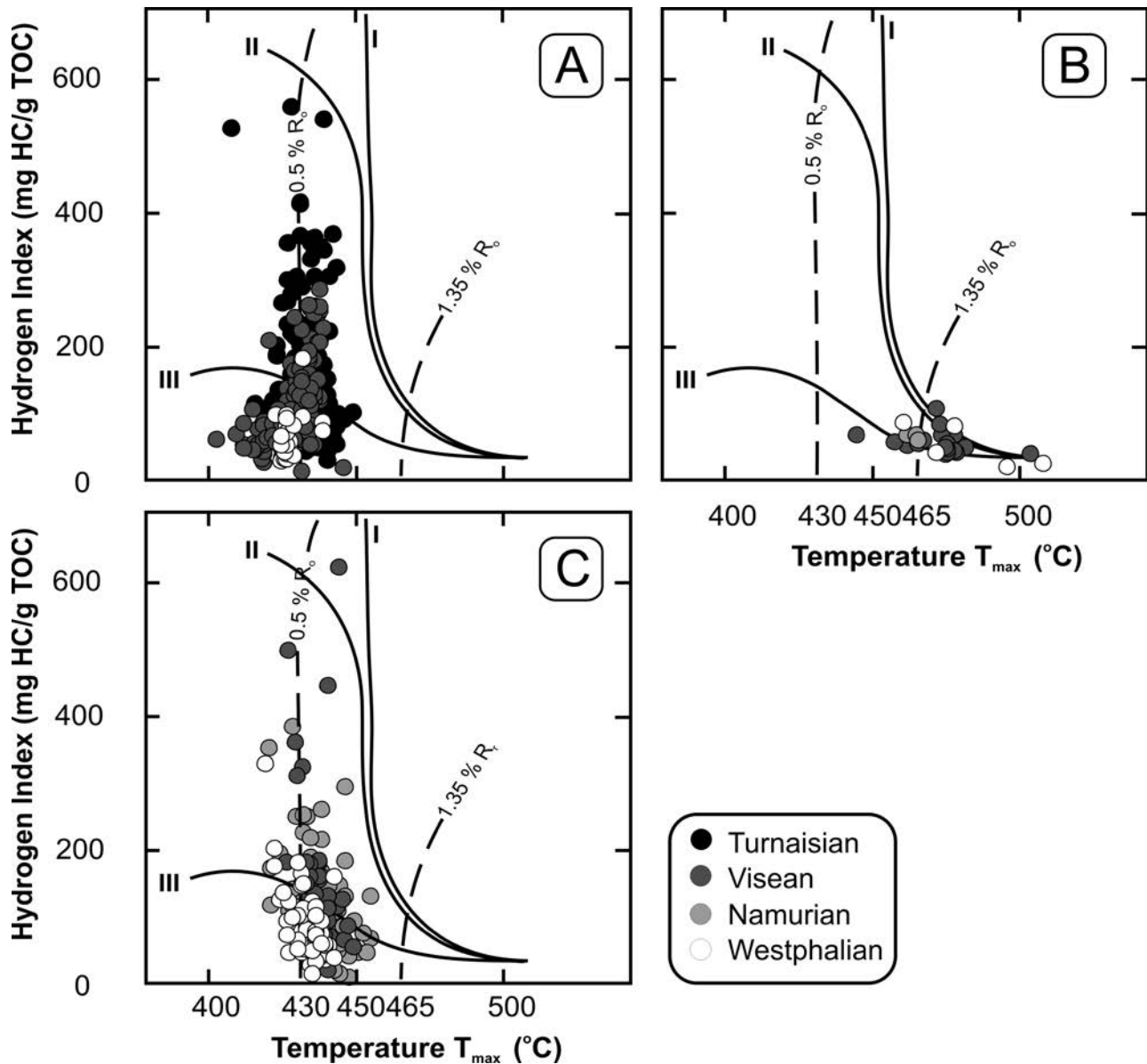
Fig. 4. Rock Eval Hydrogen Index versus temperature T_{max} for Carboniferous strata in (A) Pomerania, (B) Fore-Sudetic Homocline and (C) Masovia-Lublin area. Genetic curves for kerogen from Espitalié et al. (1985). Data modified after Bachleda-Curuś et al. (1996), Burzewski et al. (1998), Matyasik (1998), Nowak (2003), Kotarba et al. (1999, 2004, 2005), Kosakowski et al. (2006), Pletsch et al. (2010), and Poprawa (2010)
