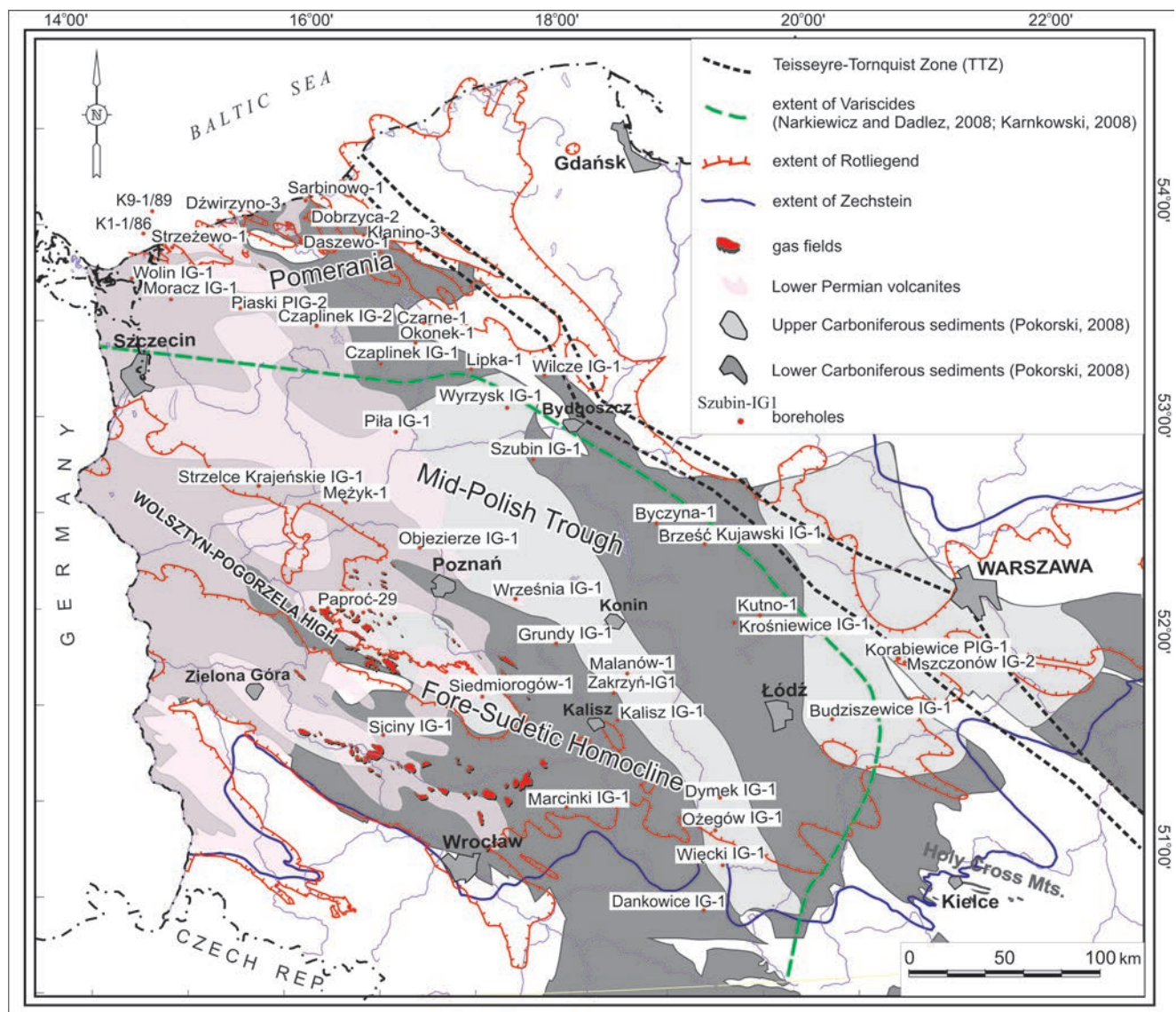
Fig. 1. Main elements of Carboniferous–Permian petroleum system in Polish Basin (based on Reicher, 2008): Carboniferous subcrop (source rocks), Rotliegend (reservoir rocks), and Zechstein (seal rock). Extent of Early and Late Carboniferous based on Pokorski (2008)
