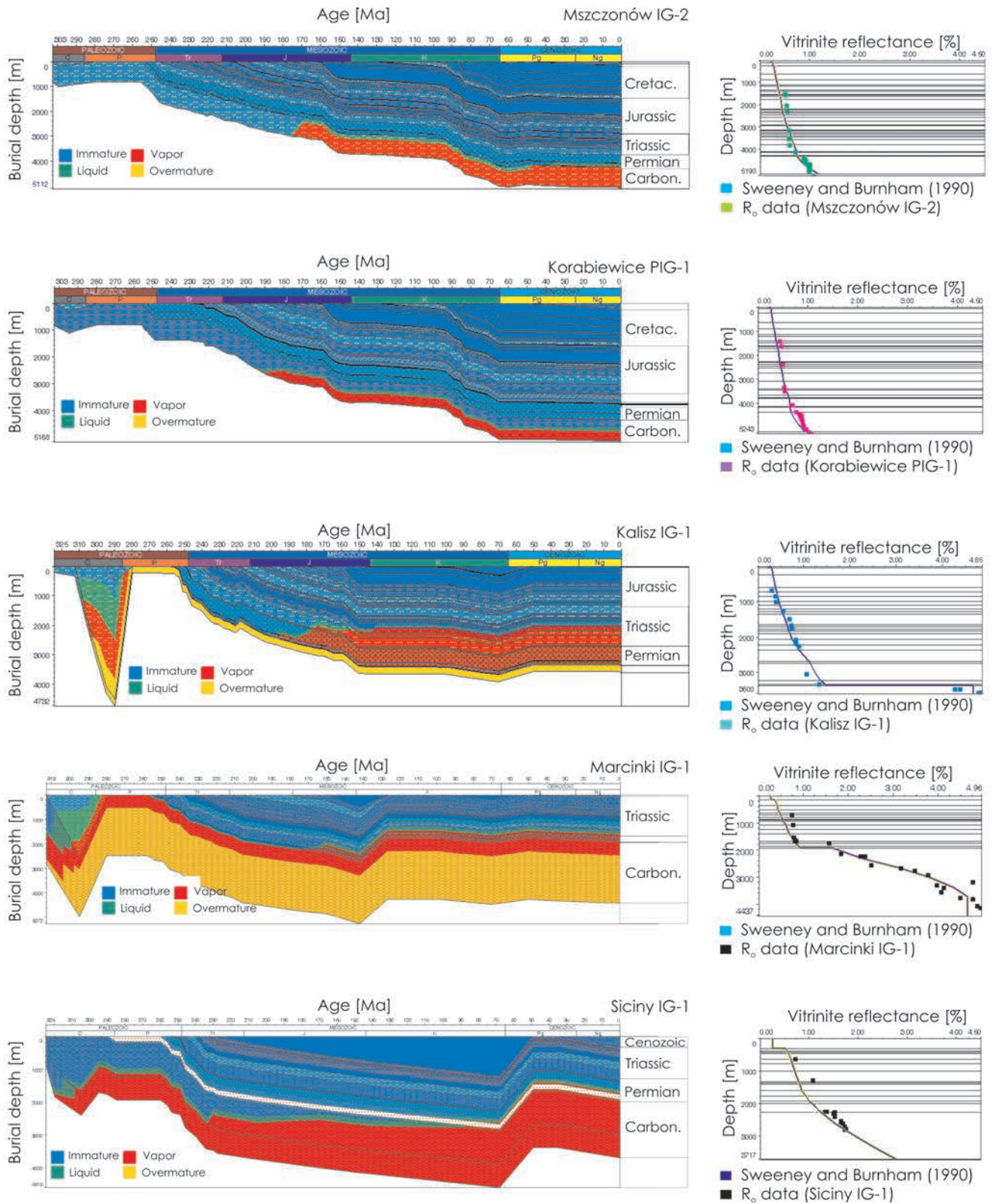
Fig. 8. Examples of selected models: Mszczonów-IG2, Korabiewice-PIG1, Kalisz-IG1, Marcinki-IG1, Sicity-IG1
