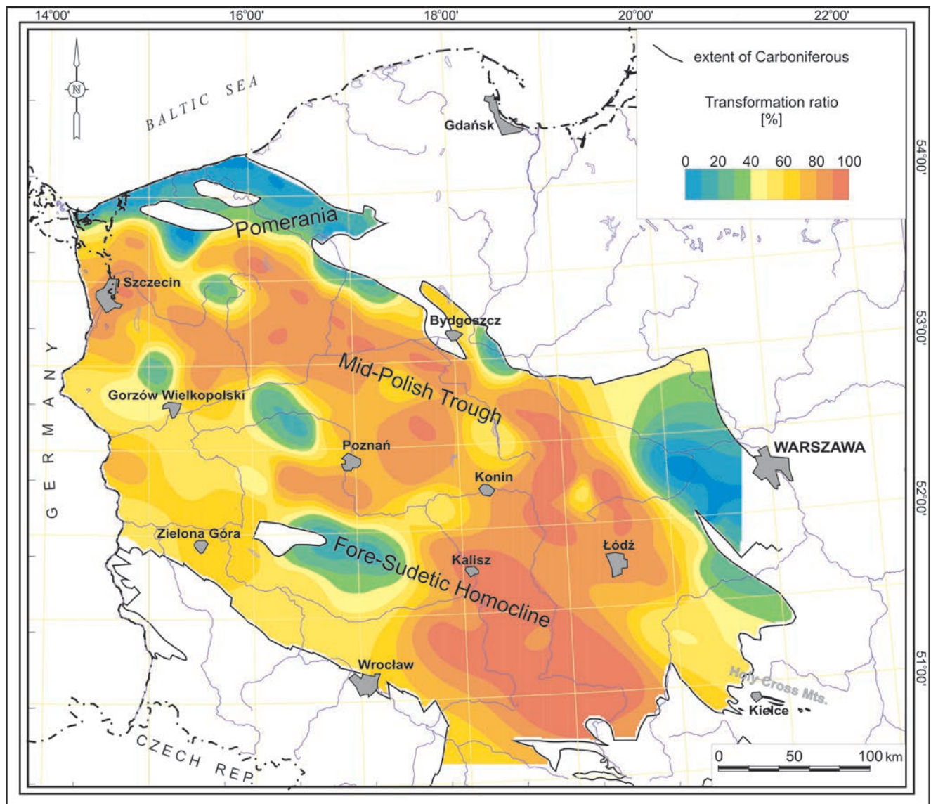
Fig. 13. Degree of kerogen transformation (TR%) in Carboniferous source rocks (referred to top of Carboniferous) calculated for the end of Triassic
