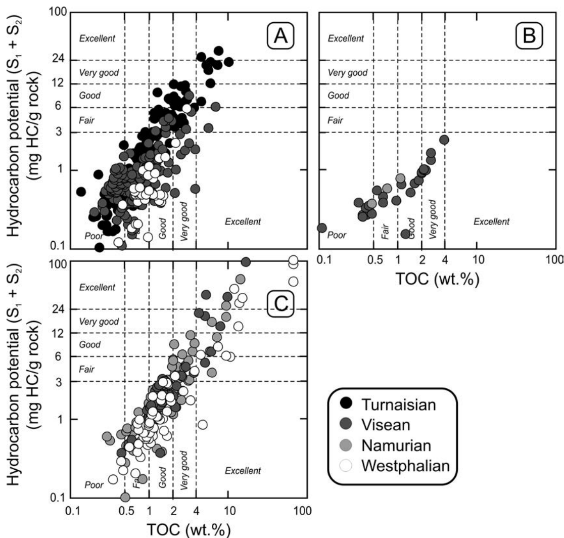
Fig. 5. Petroleum source quality diagram for Carboniferous strata in (A) Pomerania, (B) Fore-Sudetic Homocline and (C) Masovia-Lublin area. Classification after Hunt (1979) and Peters and Cassa (2002). Data modified after Bachleda-Curuś et al. (1996), Burzewski et al. (1998), Matyasik (1998), Nowak (2003), Kotarba et al. (1999, 2004, 2005), Kosakowski et al. (2006), Pletsch et al. (2010), and Poprawa (2010)
