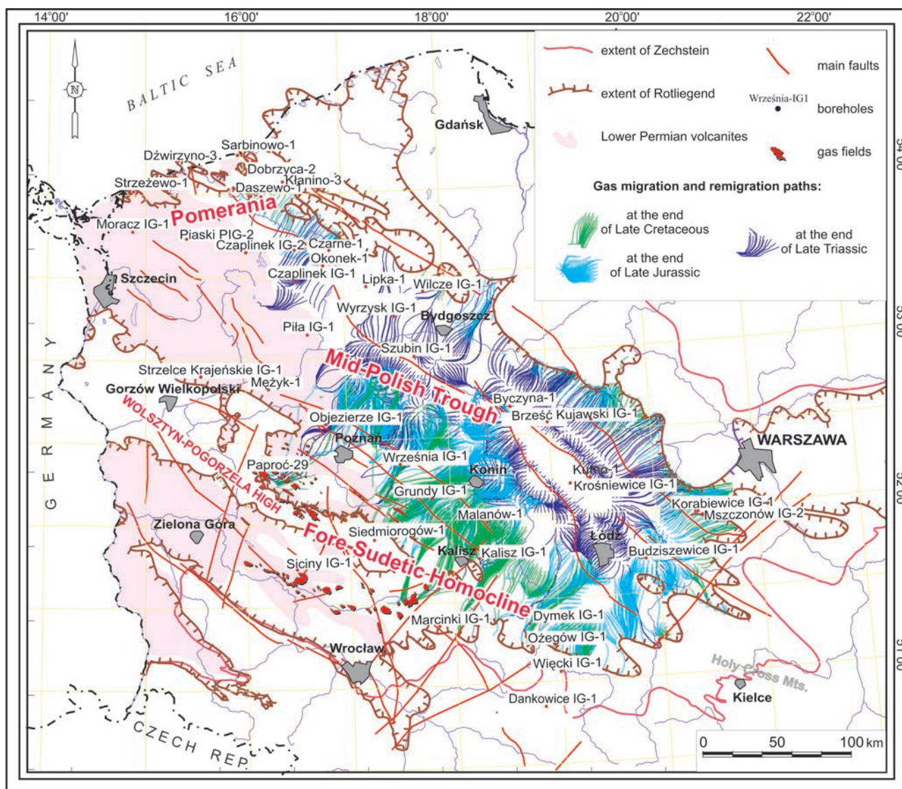
Fig. 15. Gas migration paths at top of Upper Rotliegend reservoir rocks (modified after Maćkowski et al. , 2008)
