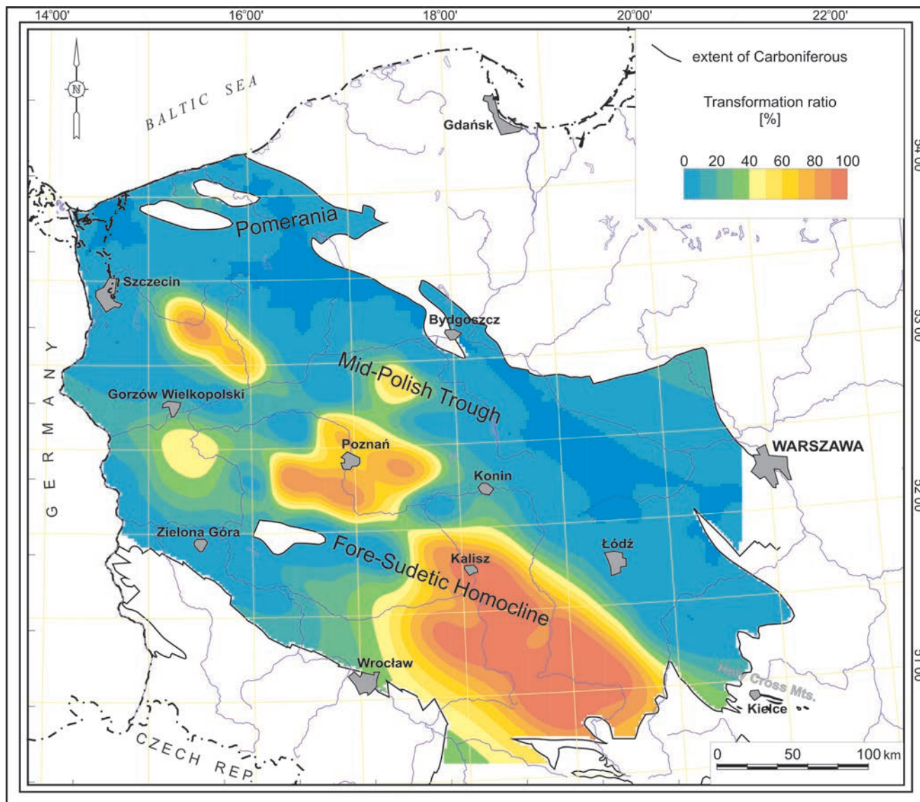
Fig. 12. Degree of kerogen transformation (TR%) in Carboniferous source rocks (referred to top of Carboniferous) calculated for end of Carboniferous
