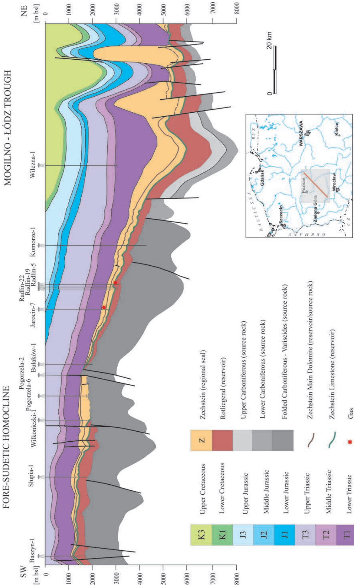
Fig. 2. Schematic cross-section across Fore-Sudetic Homocline (Cainozoic section removed; modified after Górecki, 2006; Pletsch et al. , 2010)
