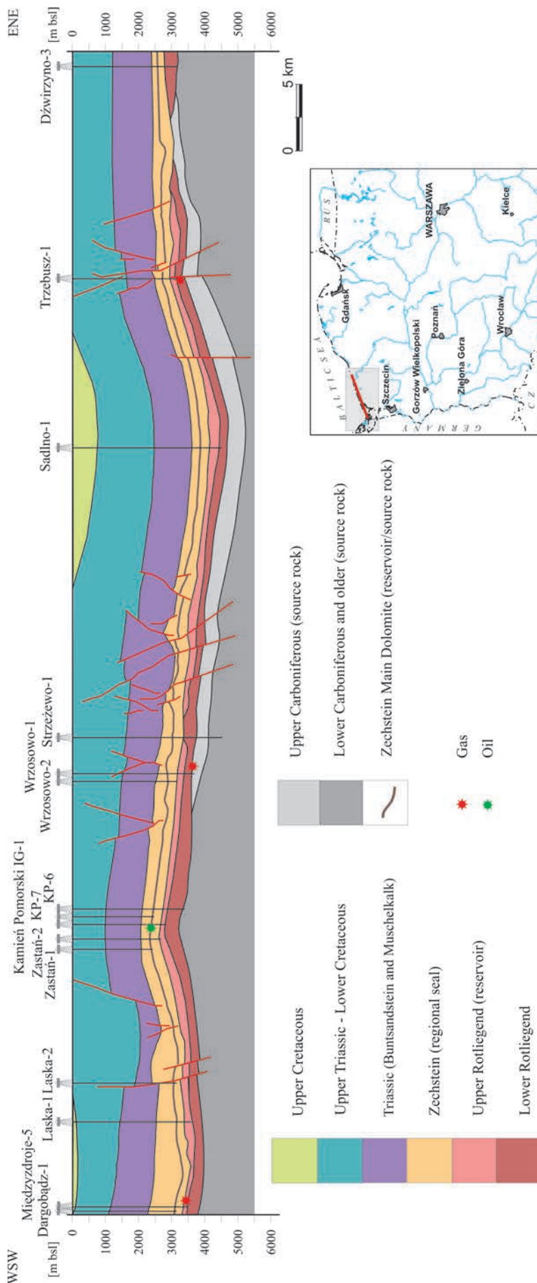
Fig. 3. Schematic cross-section across Pomerania (Cainozoic section removed; modified after Górecki, 2008; Pletsch et al. , 2010)
