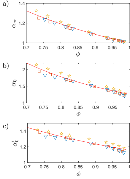
Fig. 9. Porosity-tortuosity relations of open-cell foams: high-frequency tortuosity (top), static viscous tortuosity (middle), and static thermal tortuosity (bottom). Numerical estimations are shown with Kevin pattern ( \nabla ), Waire-Phelan pattern ( \square ), and Voronoi tessellation ( \star ). The continuous lines are the fitting curves from Eq. (19).
