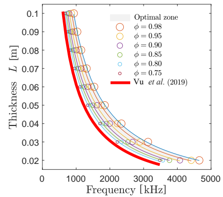
Fig. 15. Frequency at the first absorption peak of the optimal absorbers. Circle markers are the considered points, and the thin lines are the fitting exponential laws. The size of circle markers indicates an increase in the porosity of foams. The thick line presents the expression for sphere-packed media (Vu et al. , 2019).
