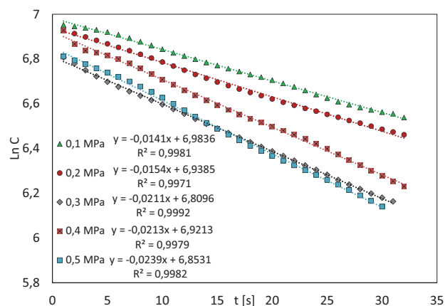
Fig. 9. Ammonia sorption curves in the kinetic range for a TF 6 V nozzle for different supply pressures
