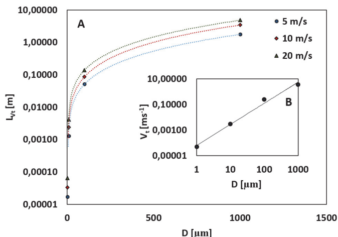
Fig. 15. A-dependence of the distance travelled by the drop ( L_{vt} ) to reach the limiting velocity ( V_t ) for the initial velocity of the droplet V_0=5, 10 and 20 \text{ ms}^{-1} .
