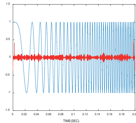
Signal plus watermark time domain diagram (a)
