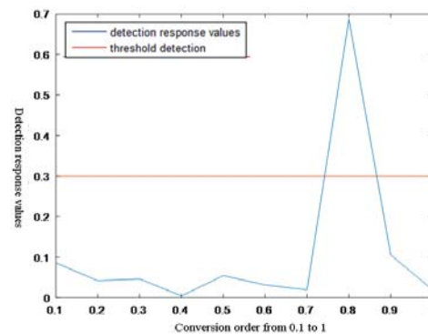
Detector response value of different order of transformation (b)
