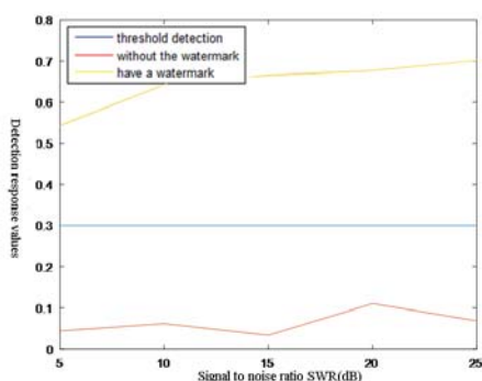
Conversion order P = 0.2 (a)
