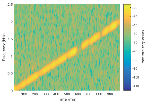
Embedded watermark plus noise (SNR = 10dB) time-frequency diagram (d)
