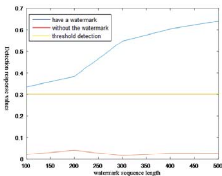
Fig.4 Detector response of different watermark length
