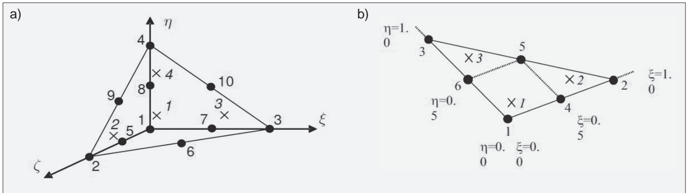
Fig. 4. Local numbering and position of nodes (•) and integration points (x) of: a) 10-node wedge element; b) 6-node plate triangle (17).
