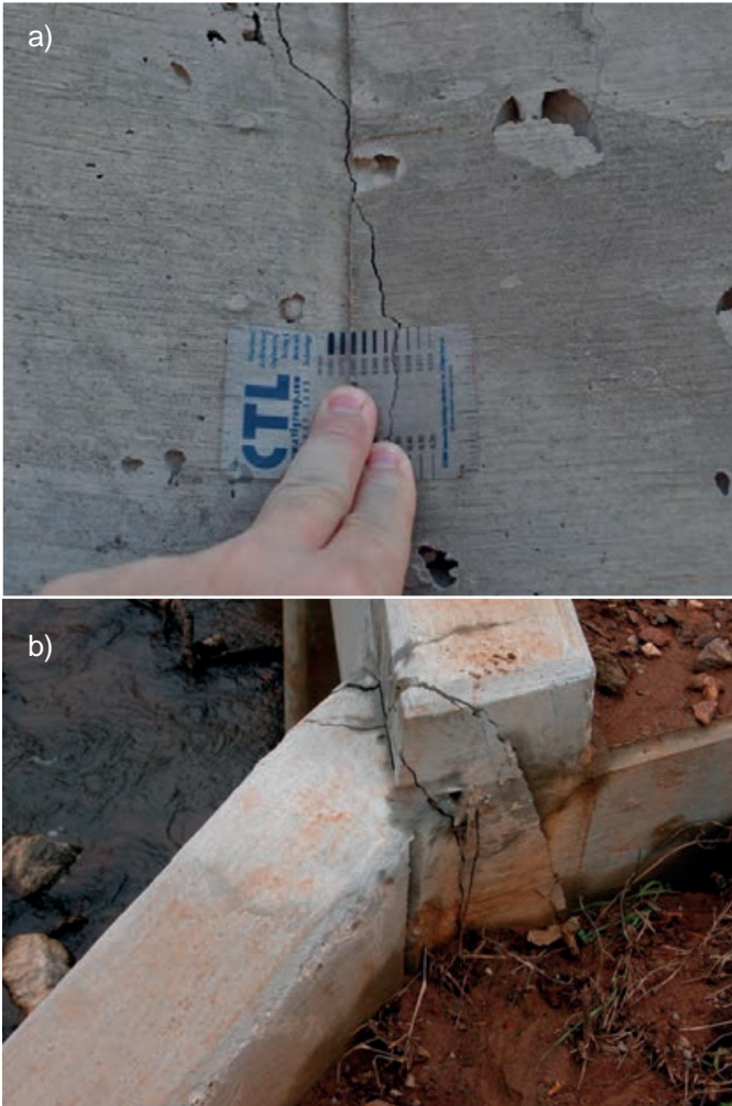
Fig. 2. Culvert distress a) Centerville, AL; b) AL 49 near Dadeville, AL.
