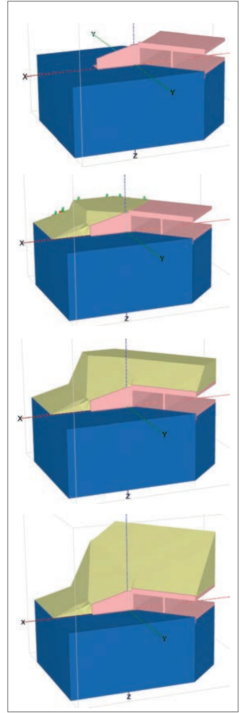
Fig. 5. Backfill construction stages.relationship in the joint*.
