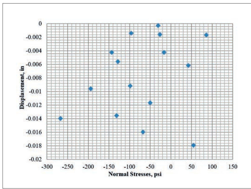
Fig. 6. Stress-displacement relationship in the joint*. *1 psi = 6.89 kN/m 2 ; 1 in. = 25.4 mm
