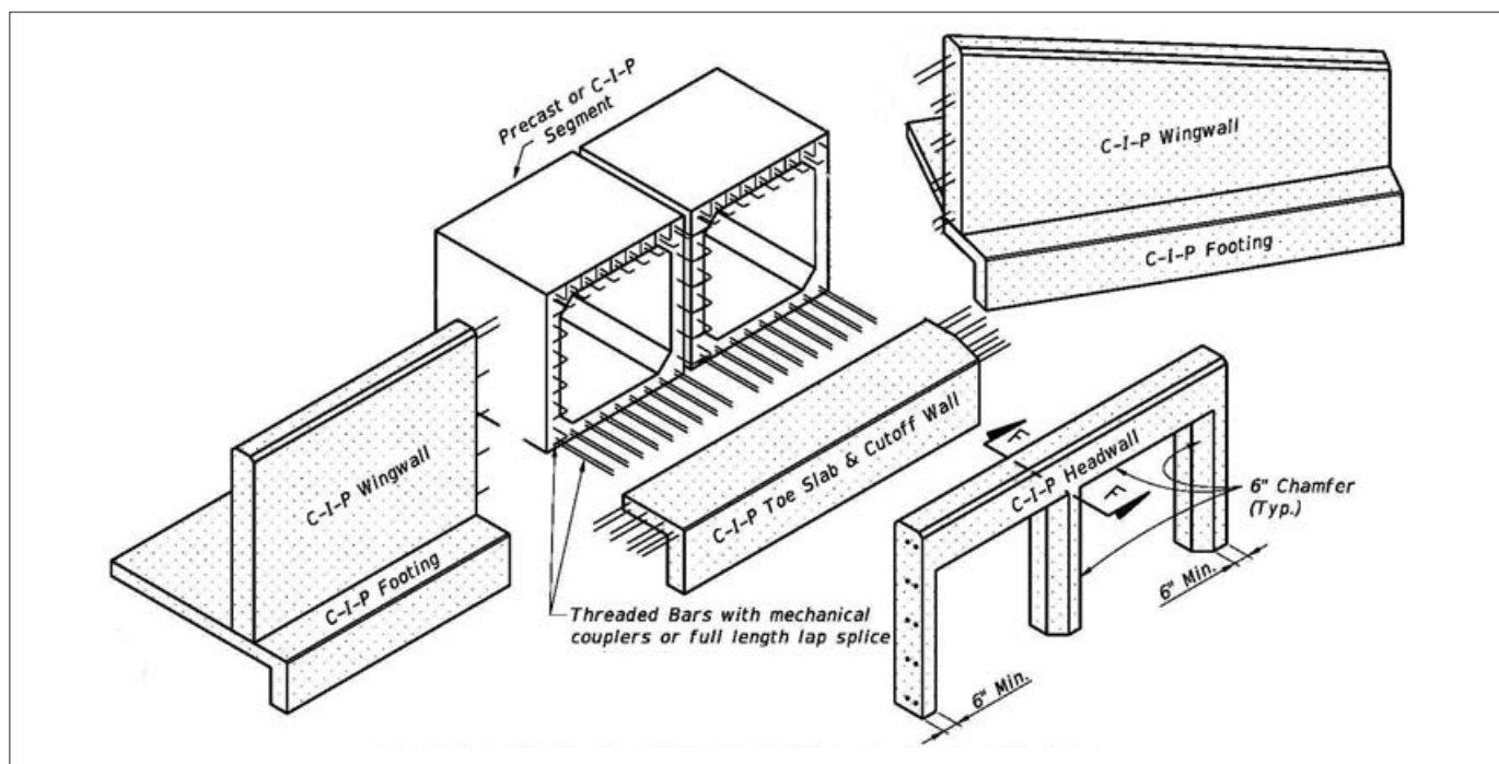
Fig. 1. General plan of the culvert (7).
