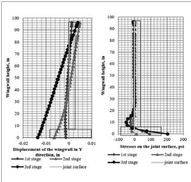
Fig. 7. Displacement and stresses along the joint height**. ** minus sign represent movement forward to the tap
