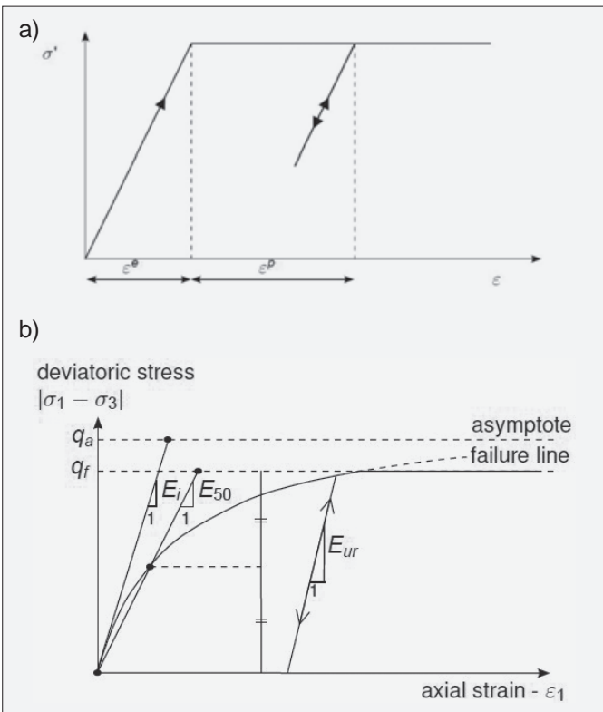
Fig. 3. Elastic perfectly plastic model (a); hyperbolic stress-strain relation (b) (14).
