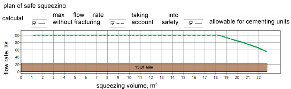
Fig. 5 Plan of safe squeezing with TSA-320
