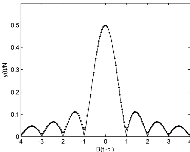
Fig. 5. Fragment of output signals around the maximal value: solid line – LFM signal, dotted line – HFM signal ( R_0 = 3 km, \tau = 4 s, f_0 = 10 kHz, B = 2 kHz, T = 10 s, f_s = 40 kHz, X_0 = 1 , M = 0 ).
