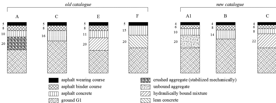
Figure 1. Pavement structure types
