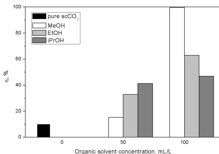
Fig. 5. The effect of organic solvent concentration on single-stage extraction efficiency \eta at 100 °C
