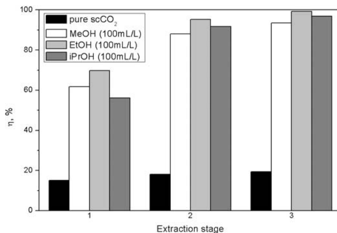
Fig. 6. Multi-stage extraction efficiency (70 °C, 18 MPa, 120 min, 100 mL/L organic solvent)
