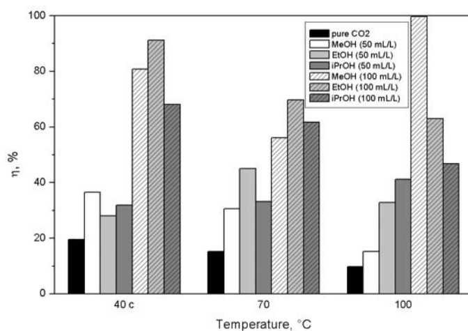
Fig. 2. The effect of temperature on single-stage extraction efficiency \eta
