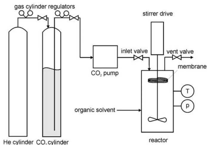
Fig. 1. Experimental setup
