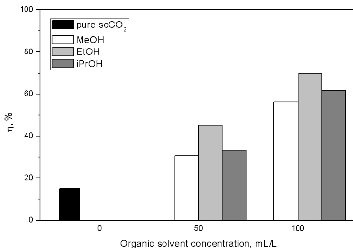
Fig. 4. The effect of organic solvent concentration on single-stage extraction efficiency \eta at 70 °C
