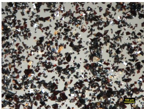
Fig. 6. Picture of the -45\ \mu\text{m} fraction of concentrate produced from single stage beneficiation process by HGMS
