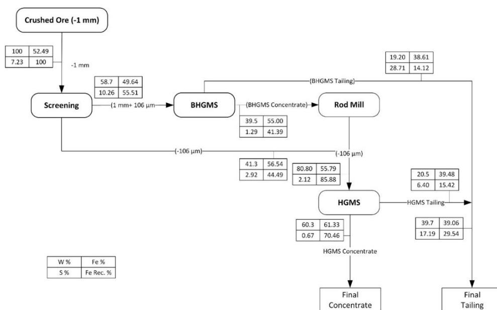
Fig. 4. Beneficiation circuit incorporating BHGMS and HGMS
