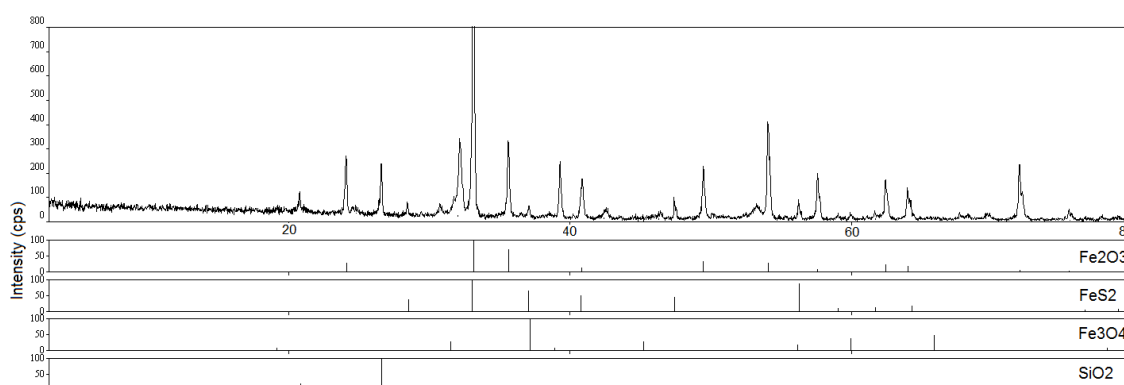
Fig. 1. XRD diffractogram of micaceous iron oxide ore
