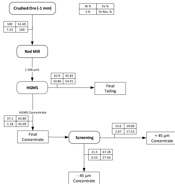
Fig. 5. Single stage beneficiation by HGMS
