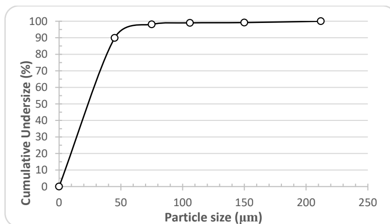
Fig. 7. Particle size distribution of the feed after grinding in pendulum ball mill
