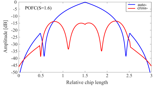
Fig. 5. COM simulation of auto- and cross-correlation of POFC ( S = 1.6 ). The time axis is normalized with chip length \tau_{\text{chip}} . The peak value of the cross-correlation is approximately -13 dB.
