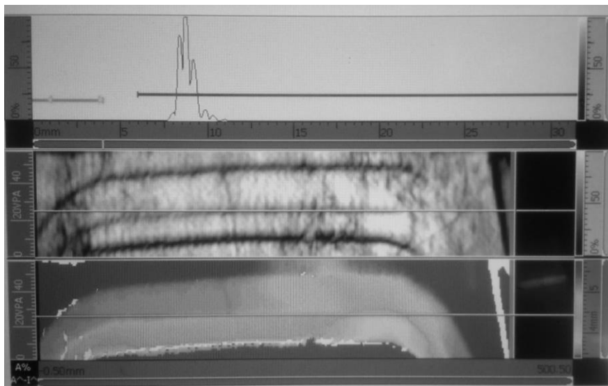
Fig. 3. A-C-C-scan views of the inspected sample
