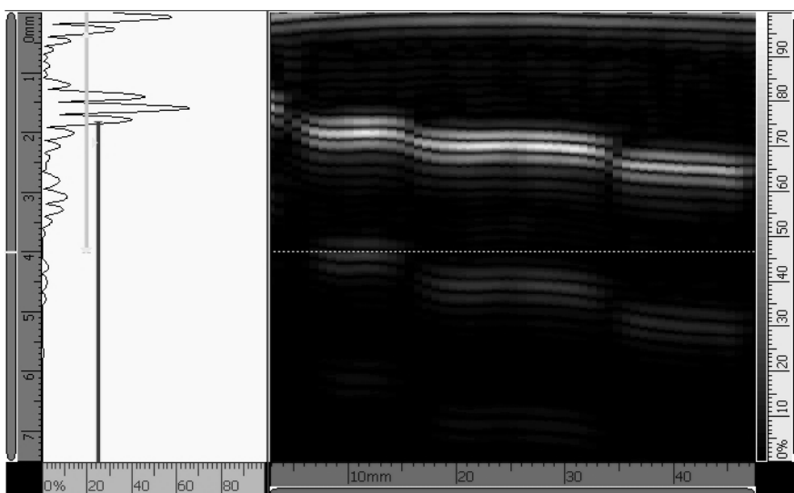
Fig. 4. A-S-scan images of the examined part of the aileron
