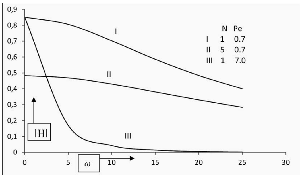
Fig.13. Amplitude |H| of the Nusselt number.
