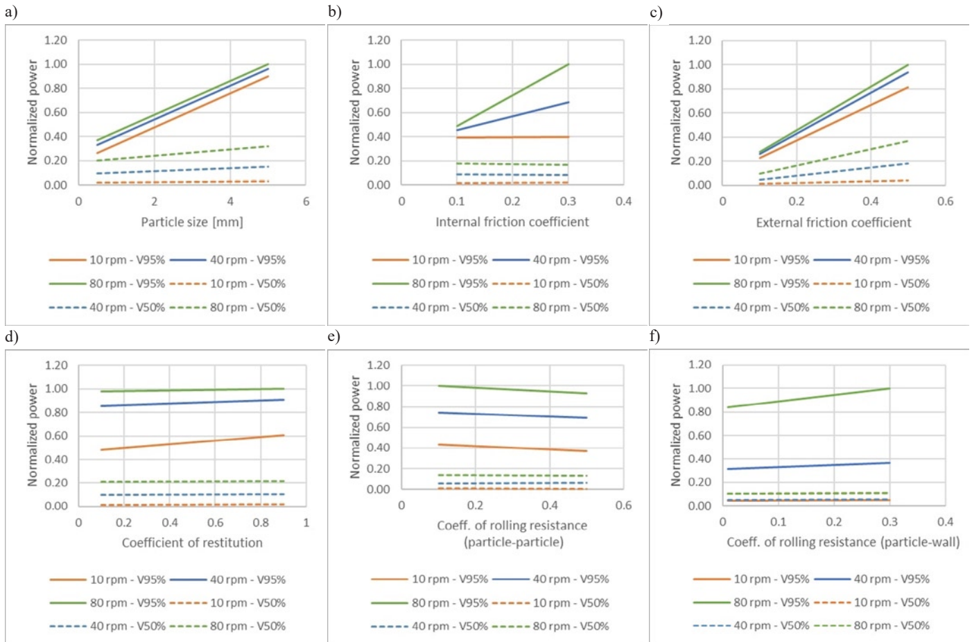
Fig. 4. The influence of the DEM model input parameters on the results of the power demand of a screw conveyor
