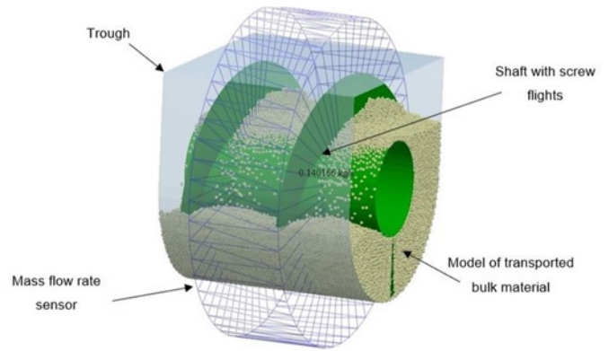
Fig. 2. A view of the modeled part of the screw conveyor.
