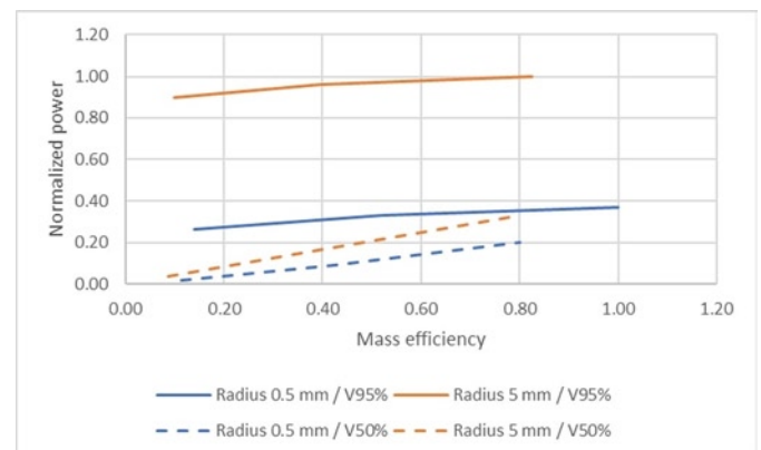
Fig. 5. The influence of the size of a DEM particle on the exploitation characteristics of a screw conveyor.
