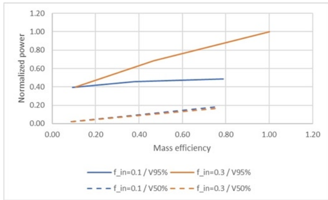
Fig. 6. The influence of the coefficient of internal friction on the exploitation characteristics of a screw conveyor
