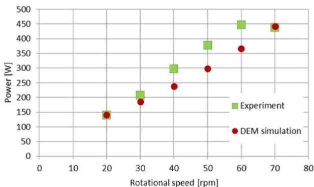
Fig. 11. The values of the power demand of the screw conveyor obtained experimentally and in the simulation as a function of the rotational speed.
