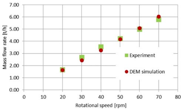
Fig. 10. The values of the mass efficiency of the screw conveyor obtained experimentally and in the simulation as a function of the rotational speed.
