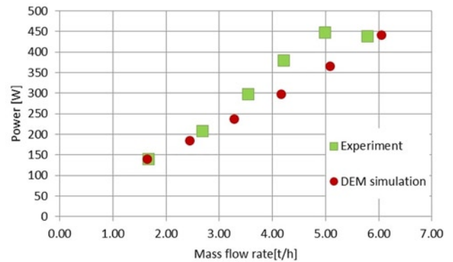
Fig. 12. Experimental and simulated exploitation characteristics of the tested screw conveyor.
