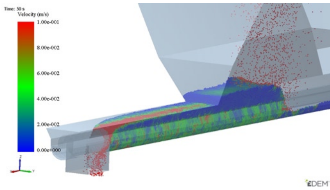
Fig. 9. Velocity distribution inside the trough of the modeled screw conveyor
