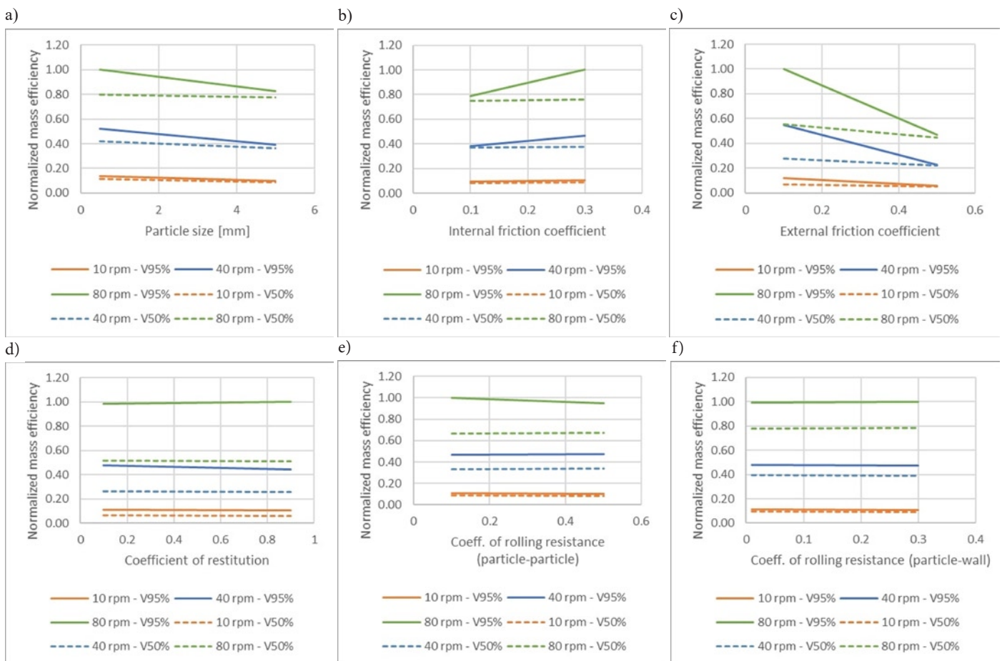
Fig. 3. The influence of the DEM model input parameters on the results of the mass efficiency of a screw conveyor.
