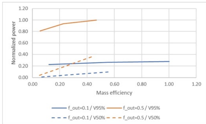
Fig. 7. The influence of the coefficient of external friction on the exploitation characteristics of a screw conveyor
