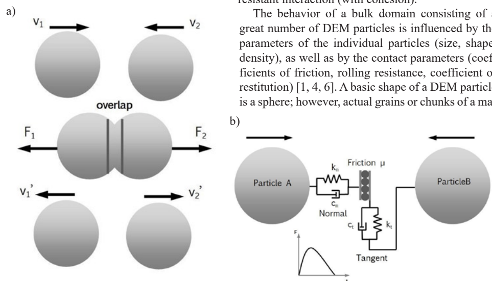
Fig. 1. a) The collision of rigid particles, where: v_1, v_2 – velocities of the particles before the collision, F_1, F_2 – forces resulting from the collision, v_1', v_2' – velocities of the particles after the collision; b) a contact model of two particles during the collision, where: k_n – stiffness modulus, normal to the surface of the contact, k_t – stiffness modulus, tangent to the surface of the contact, c_n – viscous damping coefficient, normal to the surface of the contact, c_t – viscous damping coefficient, tangent to the surface of the contact, \mu – Coulomb coefficient of friction
