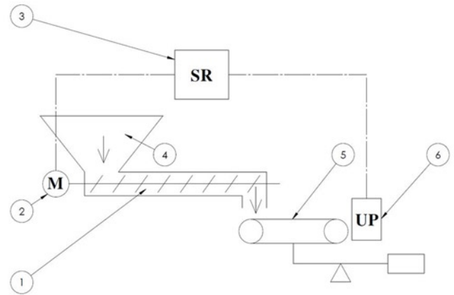
Fig. 8. A scheme of the laboratory test setup.
