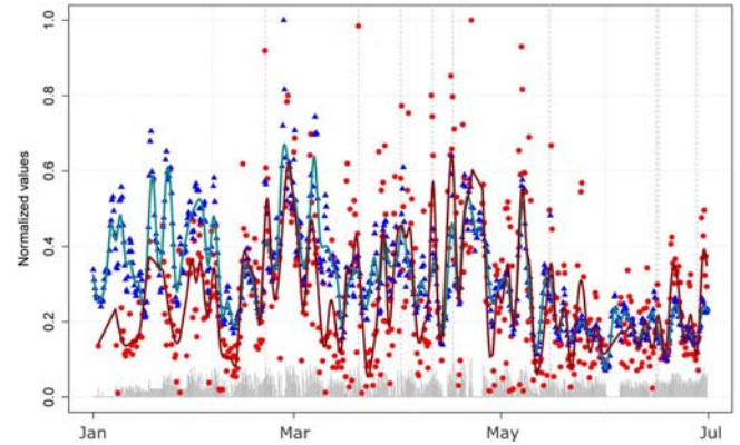
Figure 9. Normalized maximum wave height (at 4 different times a day, blue triangles) and normalized maximum rate of change in CA (at the same time period of day, red dots), together with fitted smoothing splines in the same colors (smoothing parameter 0.2). Observe the nicely visible co-variation of the smoothed signals. The gray bars at the bottom indicate the number of AIS samples available in the various time periods (max. 9700 samples/period).
