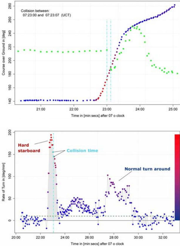
Figure 2. TOP - Course over ground (COG) for both vessels (green squares - fishing vessel, blue/red dots - ferry). Observe that the COG for the fishing vessel remained unchanged until collision, after which it changes abruptly and parallels with that of the ferry (also seen on the geo traces in Figure 1). From the changes in COG, the collision must have occurred between 7:23:00 and 7:23:07 (UCT) as indicated with the cyan dash-dotted lines. BOTTOM - Rate of turn (ROT) of the ferry in deg/min. Observe the high peak (hard starboard maneuver) right before the collision. The red and blue color bar represents high and low values of ROT respectively. For comparison, the green dashed line represents the ROT comfort limit for cruise ships traveling at 20 knots. Thus, it may not be surprising that the ferry maneuvers were experienced as slightly uncomfortable by passengers.
