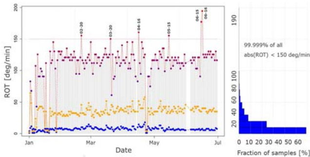
Figure 3. LEFT - The daily maximum |ROT| values (upper red dots), the daily median |ROT| values (blue dots), and the |ROT| values corresponding to the 95 % percentile (orange dots) of the ferry over half a year. Only ROT \neq 0 were taken into account. The highest ROT peak relates to the collision with the fishing vessel. The relative high peak the day before corresponds to a sharp maneuvering during the passage between a group of islands (see Figure 4). It is easy to pick out any non-normal maneuvering from this single ship time series plot. Here all |ROT| \geq 150 deg/min are tagged with the date of occurrence. RIGHT - Frequency of occurrence of various |ROT| values. Note that 99.999 % of all |ROT| \leq 150 deg/min.
