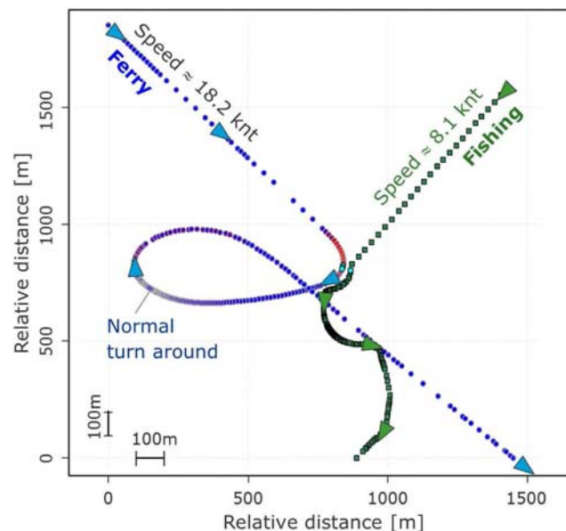
Figure 1. Visualization based on high resolution AIS data, overlaid with the low resolution AIS data points (blue triangle - ferry, green triangle - fishing vessel). Note that the ferry's low resolution AIS point at the "normal turn around" could be mistaken as an outlier. The high resolution trace of the ferry is color coded according to its rate of turn (blue low ROT, red high ROT). The collision points in their traces are indicated with cyan dots.
