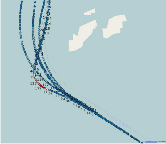
Figure 4. AIS track of a ferry navigating through a group of small islands. The track has been color coded according to the rate of turn (blue - low ROT, red - high ROT). Note the very large ROT values of the lowermost track compared to the more normal values on previous passages around the islands.
