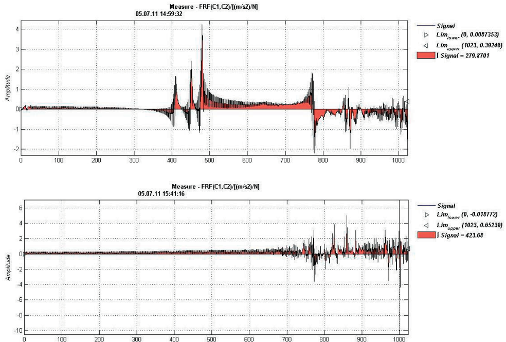
Fig.8. Realistic FRF signals form an impact test of wall bricks
