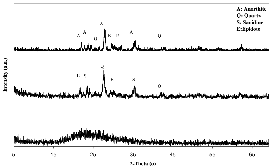
Fig. 2. XRD patterns of the samples
