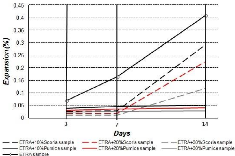
Fig. 3. Mortar-Bar test results showing the effect of percentage of pumice and scoria aggregate on expansion and time
