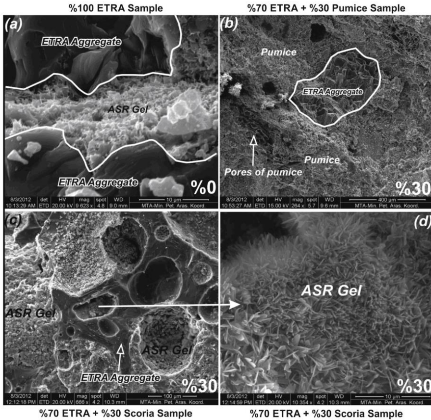
Fig. 4. SEM photomicrographs of the original and 30% pumice and scoria added samples
