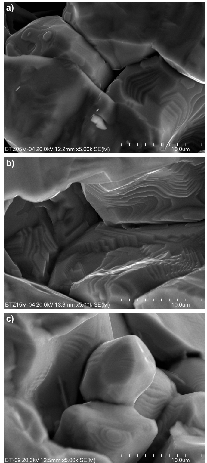
Fig. 4. SEM micrographs of the fractured surface of samples BTZ05 (a), BZT15 (b) and BT (c); magn. 5 000 \times
