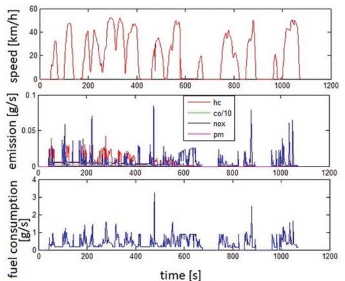
Fig. 6. Results of simulations of a hybrid drive unit with battery capacity of 8.8 kWh for the test drive at 3:00-4:00 P.M.
