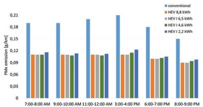
Fig. 8. PMx emission during test drives at specific times of day
