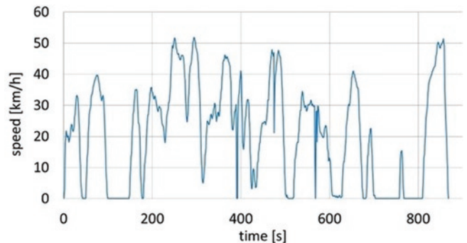
Fig. 3. Exemplary speed profile recorded during a test drive between 7:00 and 8:00 A.M.
