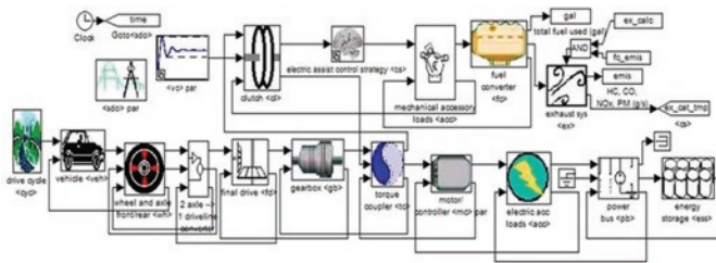
Fig. 4. Model of parallel hybrid vehicle in ADVISOR
