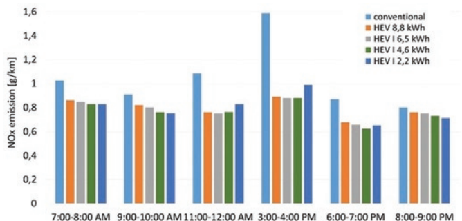
Fig. 10. NO x emission during trips at specific times of day
