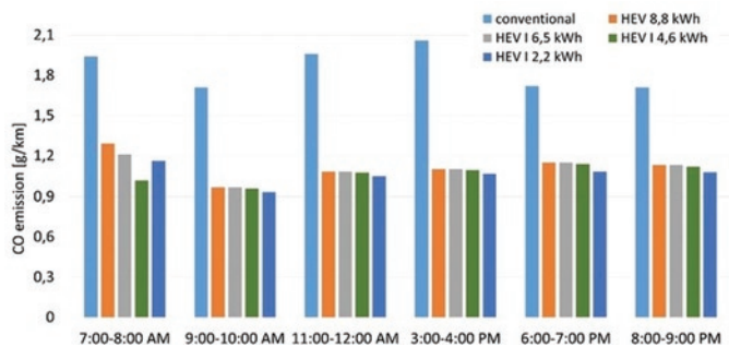
Fig. 9. CO emission during trips at specific times of day
