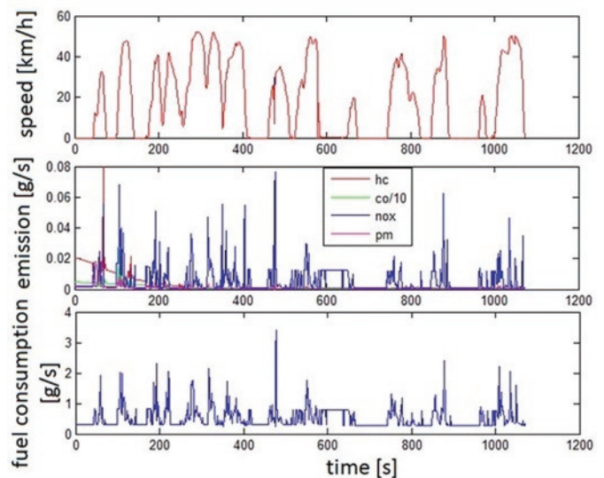
Fig. 5. Results of simulations of a conventional drive unit for the test drive at 3:00-4:00 P.M.
