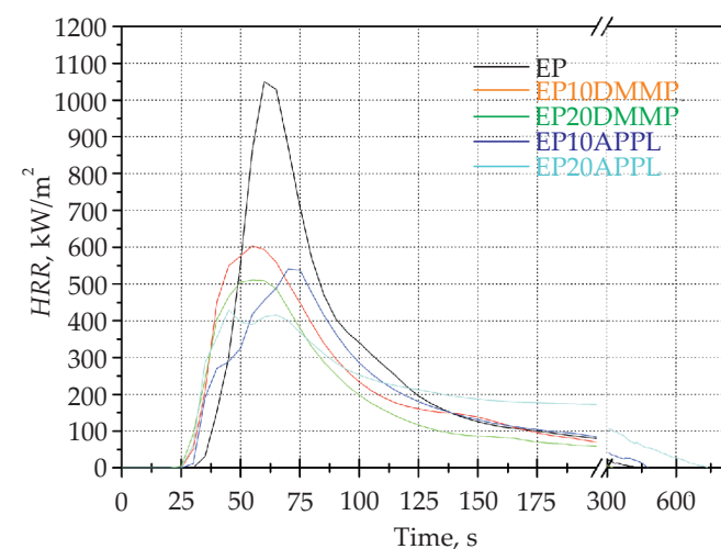
Fig. 1. Heat release rate ( HRR ) curves as a function of time during flammability tests performed in the mass loss calorimeter of unfilled epoxy resin and epoxy composites
