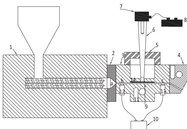
Fig. 1. The scheme of the designed extrusion head: 1 – extruder, 2 – coupling head, 3 – upper split case, 4 – die, 5 – sonotrode-transducer support, 6 – sonotrode, 7 – transducer, 8 – ultrasonic generator, 9 – rectangular profile channel, 10 – measurement chain, 11 – lower split case, 12 – sensor located before ultrasounds application area (b), 13 – sensor located after ultrasounds application area (c), 14 – separation sheet, a – location of the extrusion pressure sensor
