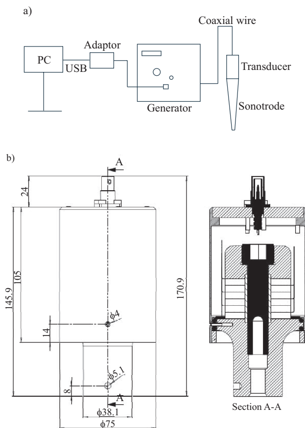
Fig. 4. Scheme of the ultrasounds device: a) block diagram, b) transducer
