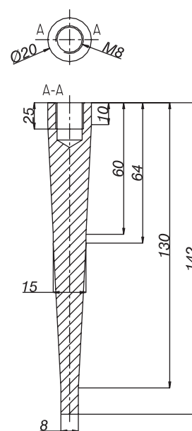
Fig. 2. Design of the sonotrode
