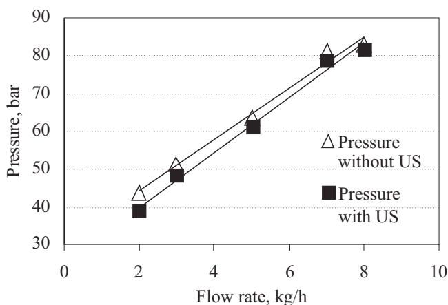
Fig. 8. Pressure dependence on flow rate measured just after the ultrasounds (US) application area
