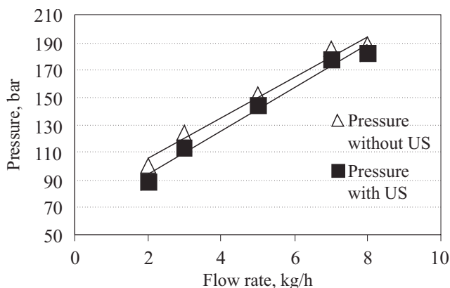
Fig. 7. Pressure dependence on flow rate measured just before the ultrasounds (US) application area
