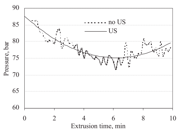
Fig. 5. Extrusion pressure with US and without ultrasounds (no US) application, along the time for extrusion with flow rate of 3 kg/h
