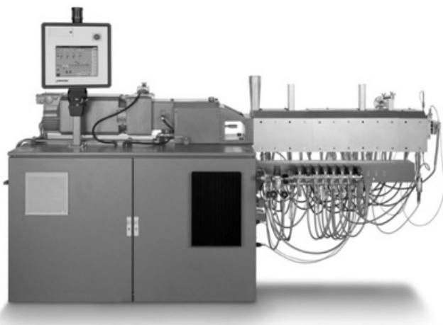
Fig. 3. Extruder Coperion ZSK 26 Mc used for experimental
