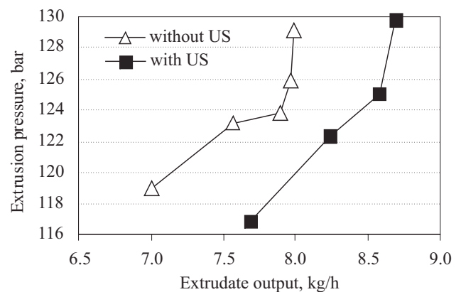
Fig. 9. Maximum flow rate reached by the extruder with and without ultrasounds (US) application under limit pressure conditions of 130 bar
