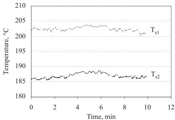
Fig. 6. Flow temperature with ultrasounds (US – continuous line) and without ultrasounds (no US – dotted line), downstream ( T_{s2} ) and upstream ( T_{s1} ) from the application area for extrusion with flow rate of 3 kg/h
