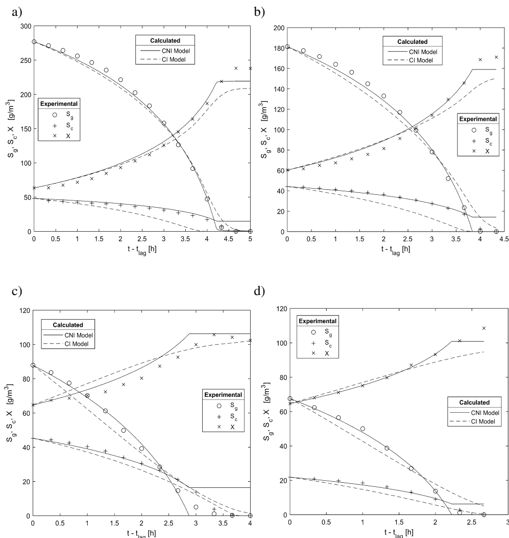
Fig. 6. Experimental and calculated profiles of 4-CP, phenol and biomass concentration: a) S_g^0 = 276.8 g/m^3 , S_c^0 = 48.4 g/m^3 , t_{lag} = 1 h ; b) S_g^0 = 181.8 g/m^3 , S_c^0 = 44.2 g/m^3 , t_{lag} = 1 h ; c) S_g^0 = 88.6 g/m^3 , S_c^0 = 43.95 g/m^3 , t_{lag} = 0.667 h ; d) S_g^0 = 67.6 g/m^3 , S_c^0 = 21.9 g/m^3 , t_{lag} = 0.667 h
